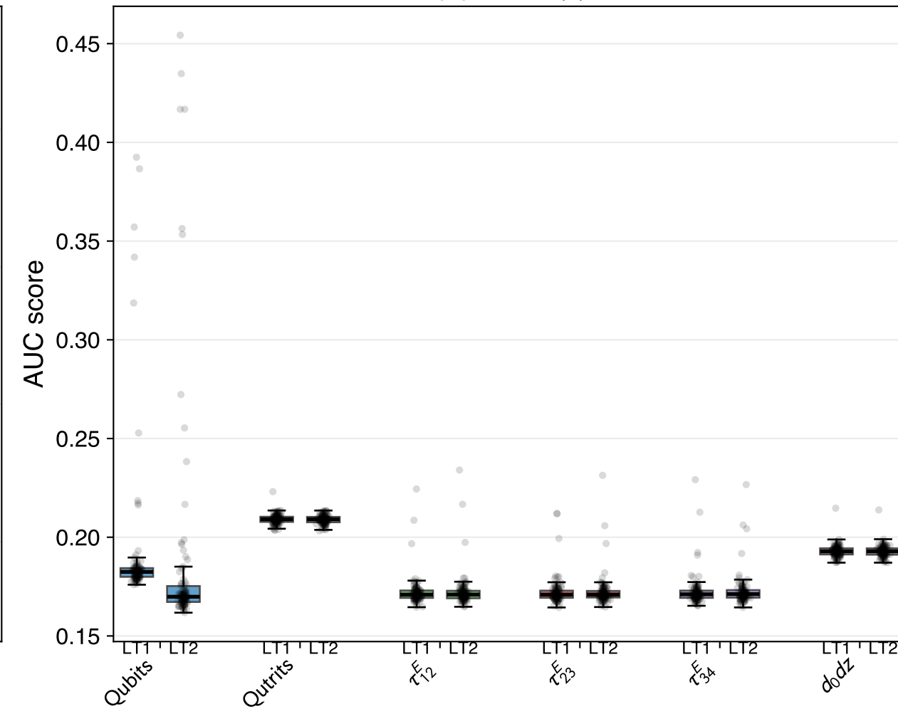
(c) t \rightarrow bq\bar{q}
