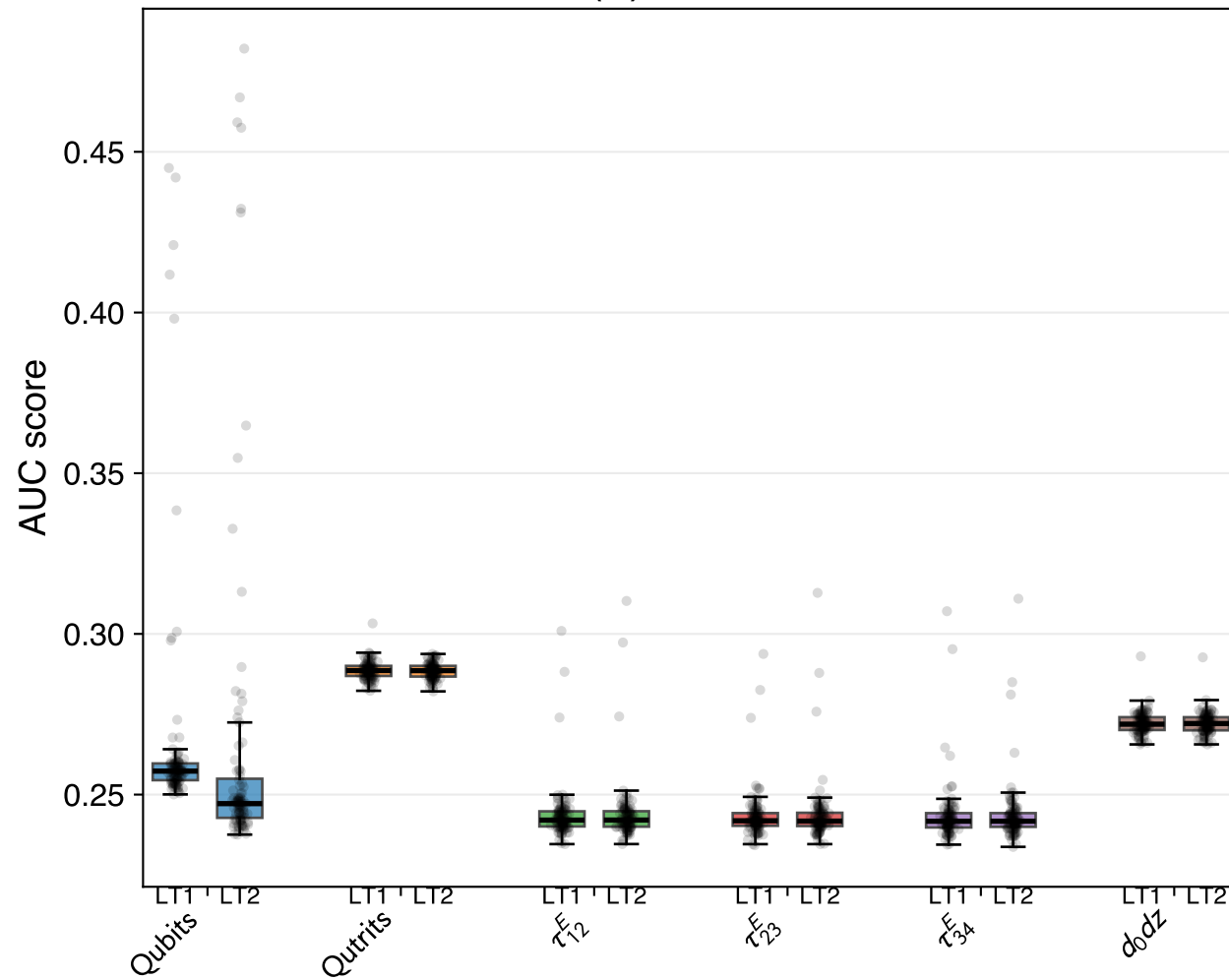
(a) H \rightarrow b\bar{b}
