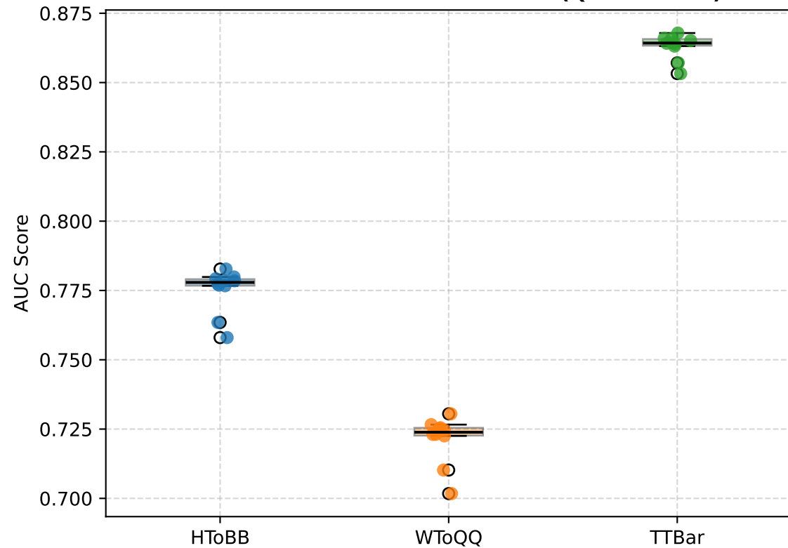
AUC Distribution Across 10 Runs (Qubits10 It2)
