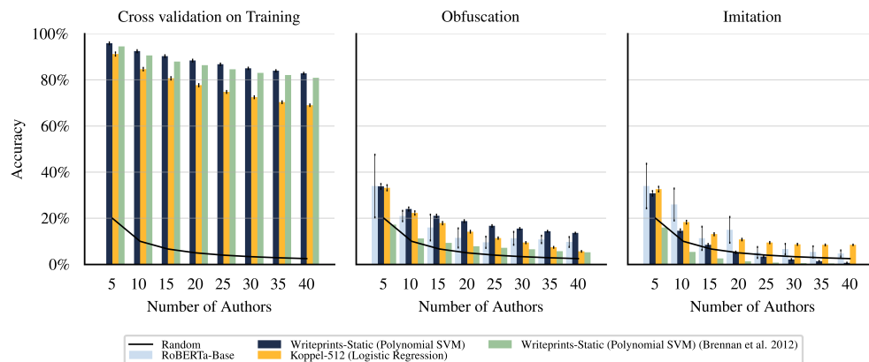
Figure 1: Reproduction of the adversarial stylometry experiment in Brennan et al. (2012). The left panel shows the accuracy of a 10-fold cross-validation using the training data. The middle and right panels indicate the accuracy of the classifier when the indicated authorship attribution circumvention strategy is used. Each bar indicates the mean accuracy; error bars show 95% confidence intervals. 10-fold cross-validation is not performed with the RoBERTa model.
