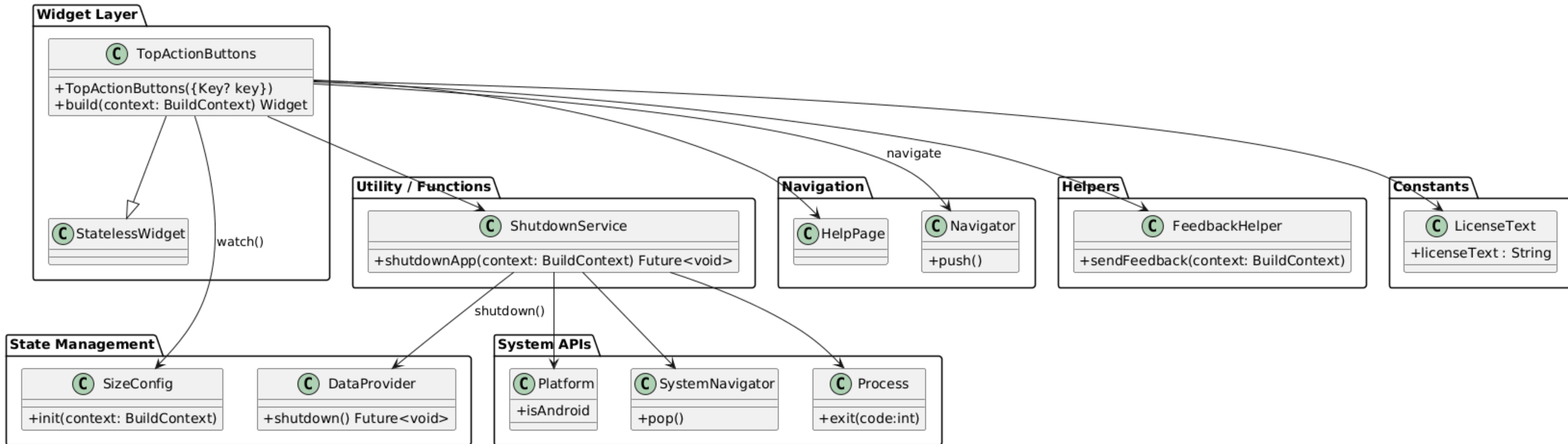
Flutter Widget Class Diagram - TopActionButton
