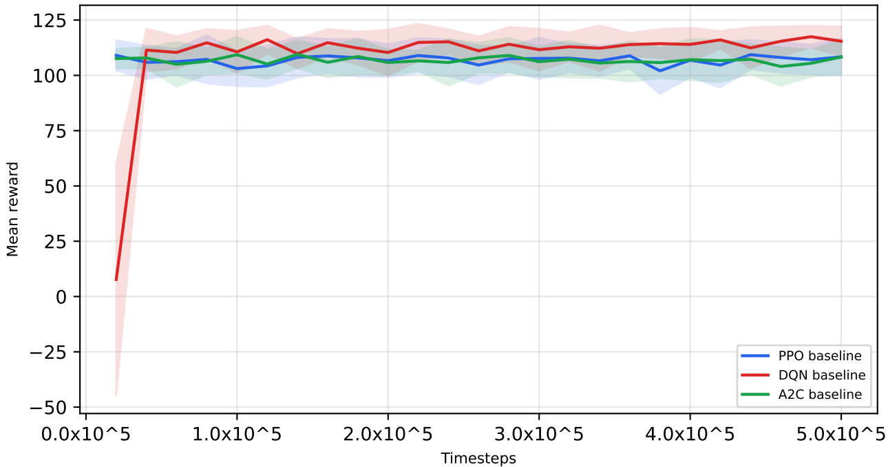
Group A -- Algorithm Comparison (lam=3.0, standard reward)
