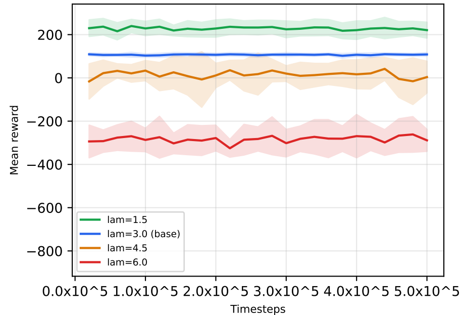
PPO -- Arrival-Rate Sweep
