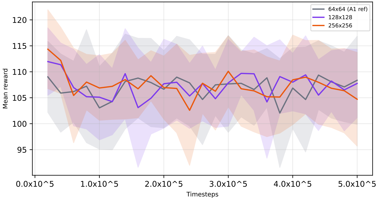
Group E -- PPO Network Architecture
