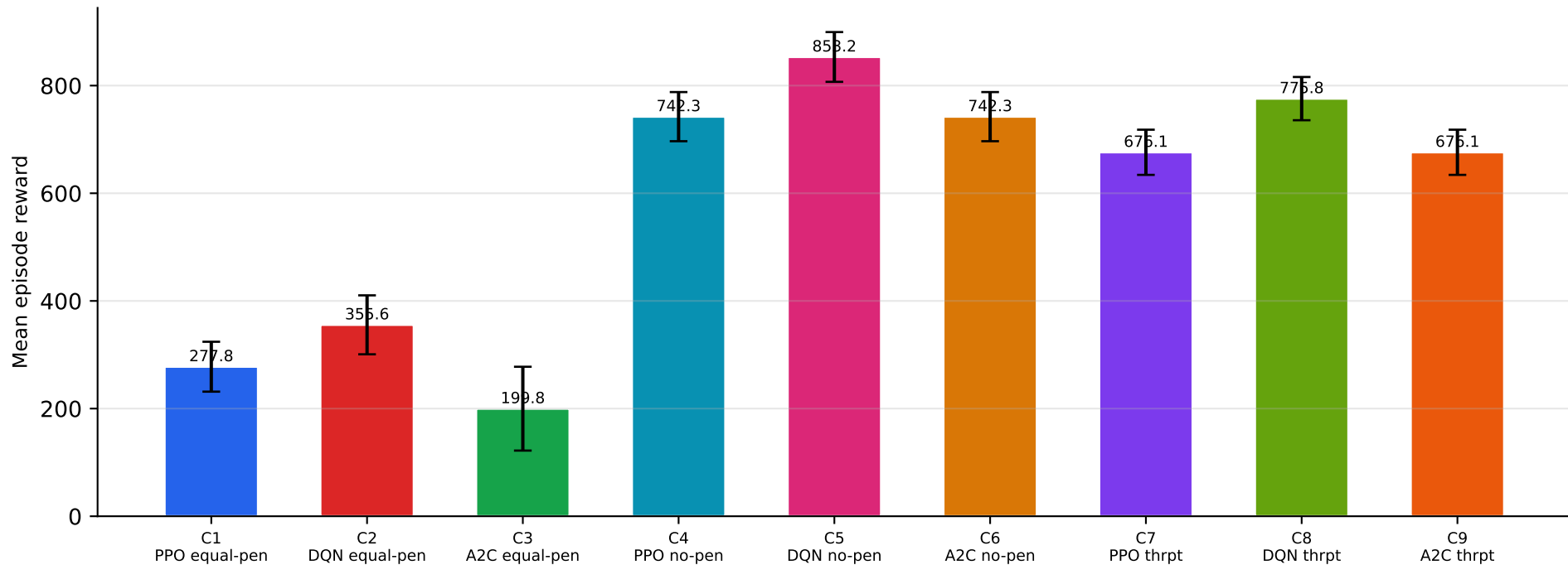
Group C — Reward-Shaping Ablation (Mean Reward)
