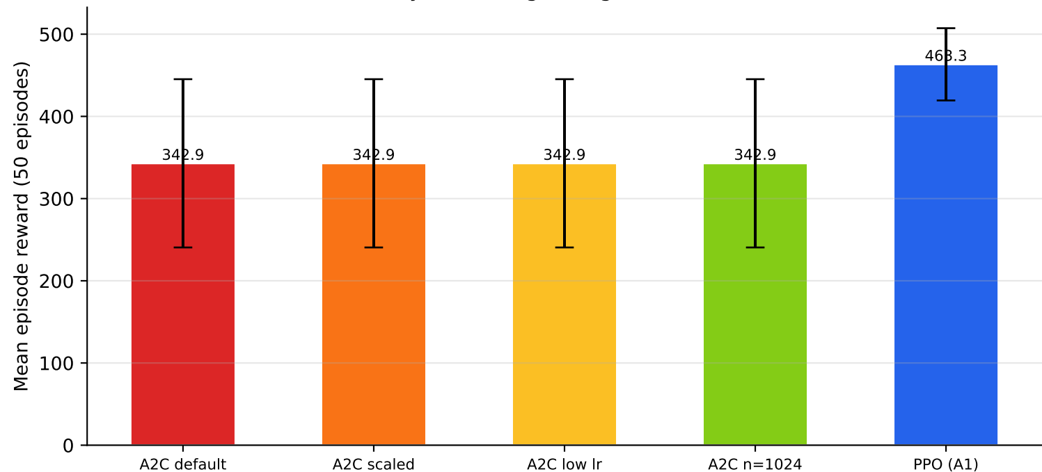
A2C Failure Analysis — Diagnosing Poor Performance vs PPO
