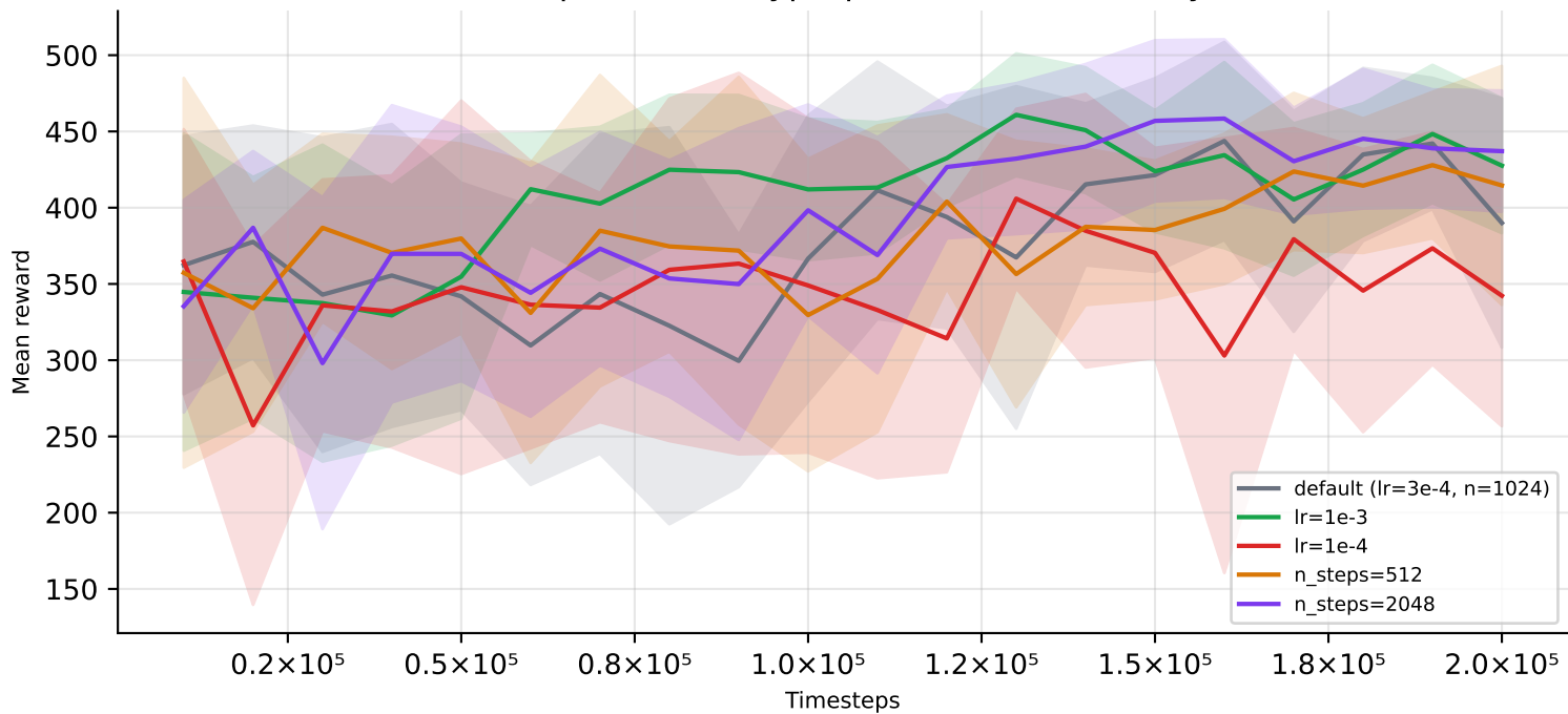
Group F — PPO Hyperparameter Sensitivity
