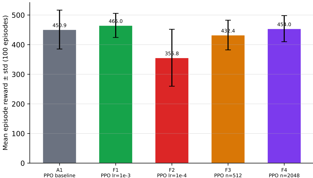
Group F — PPO Hyperparameter Sensitivity
