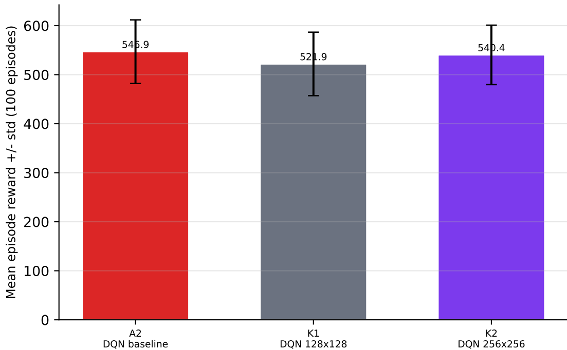
Group K -- DQN Network Architecture ( \lambda=3.0 )
