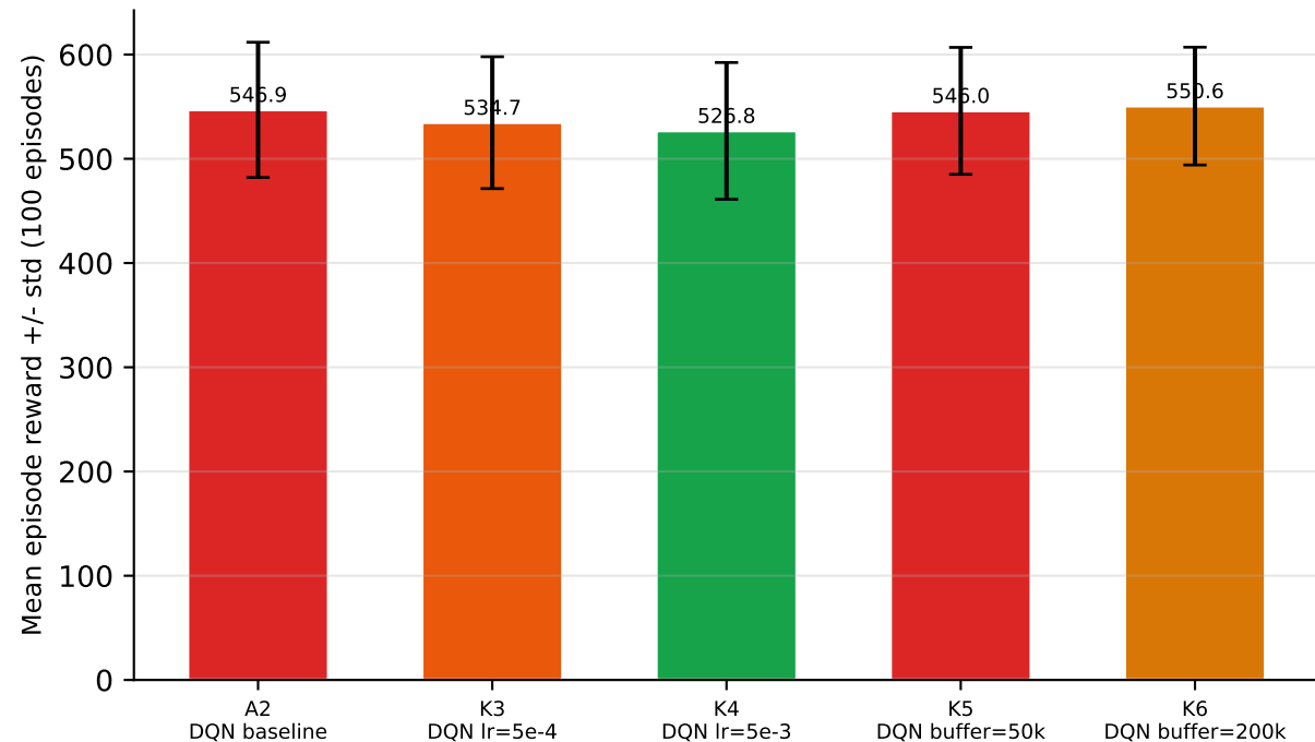
Group K -- DQN Learning Rate / Replay Buffer Sensitivity ( \lambda=3.0 )
