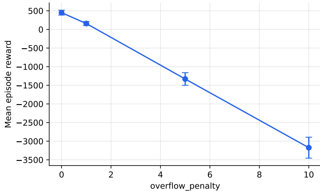
Reward vs penalty scale (PPO, \lambda=3.0 )
