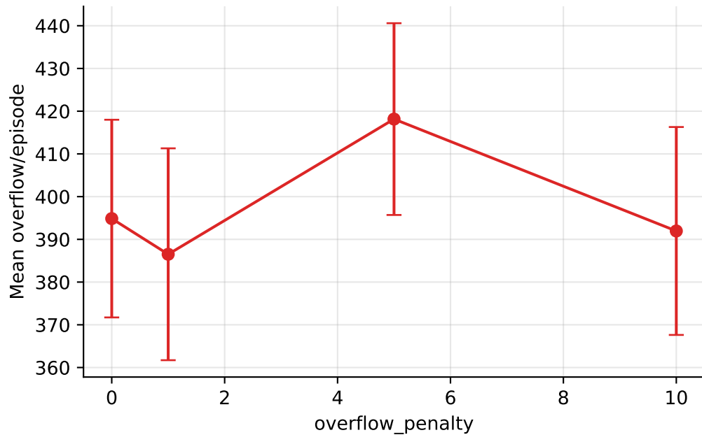
Overflow count vs penalty scale (PPO, \lambda=3.0 )
