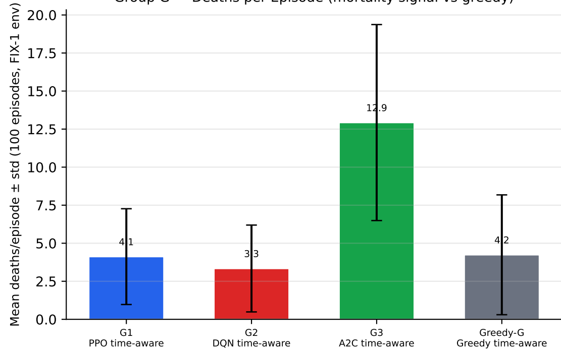
Group G — Deaths per Episode (mortality signal vs greedy)
