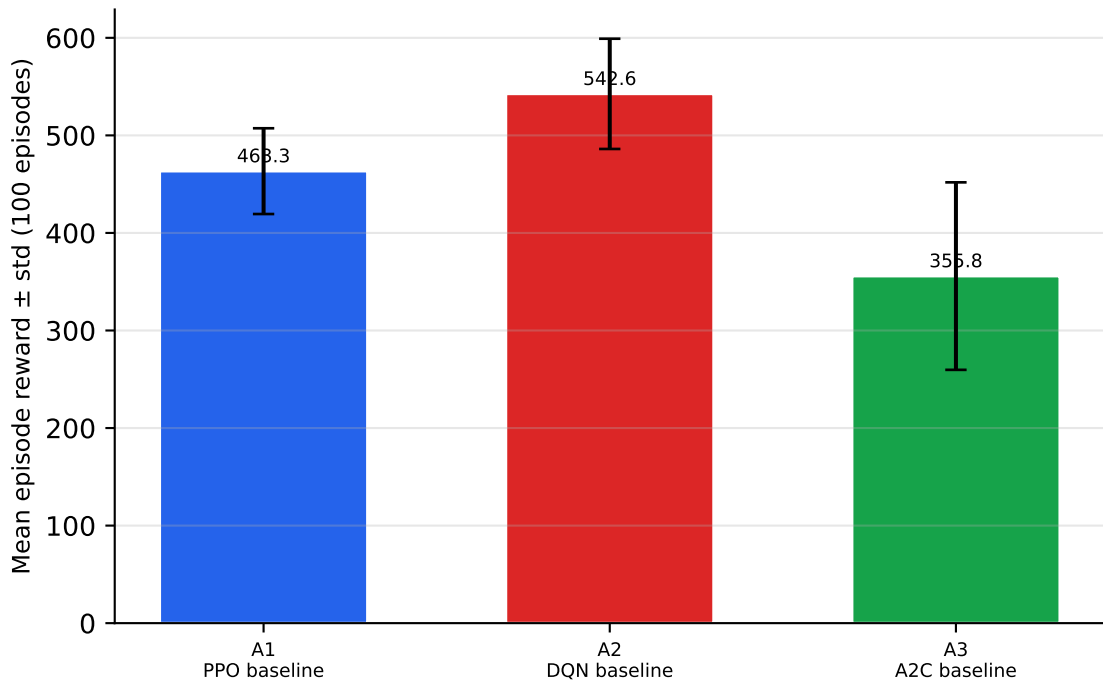
Group A — Mean Episode Reward (PPO vs DQN vs A2C)
