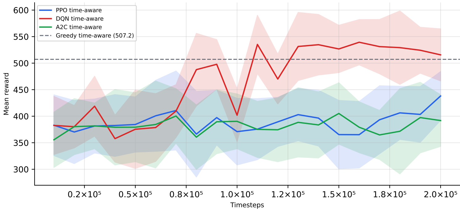
Group G — Time-Aware Reward ( \lambda=3.0 , mortality enabled)
