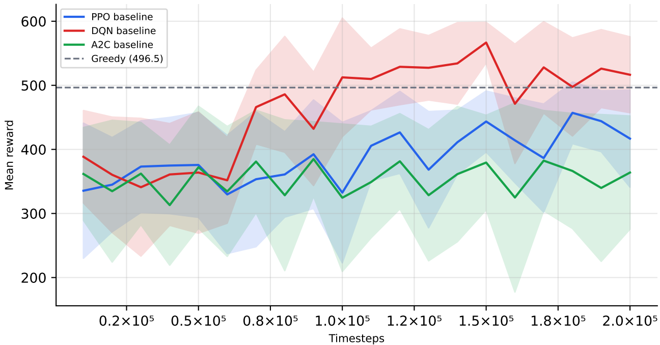
Group A — PPO vs DQN vs A2C Learning Curves ( \lambda=3.0 )
