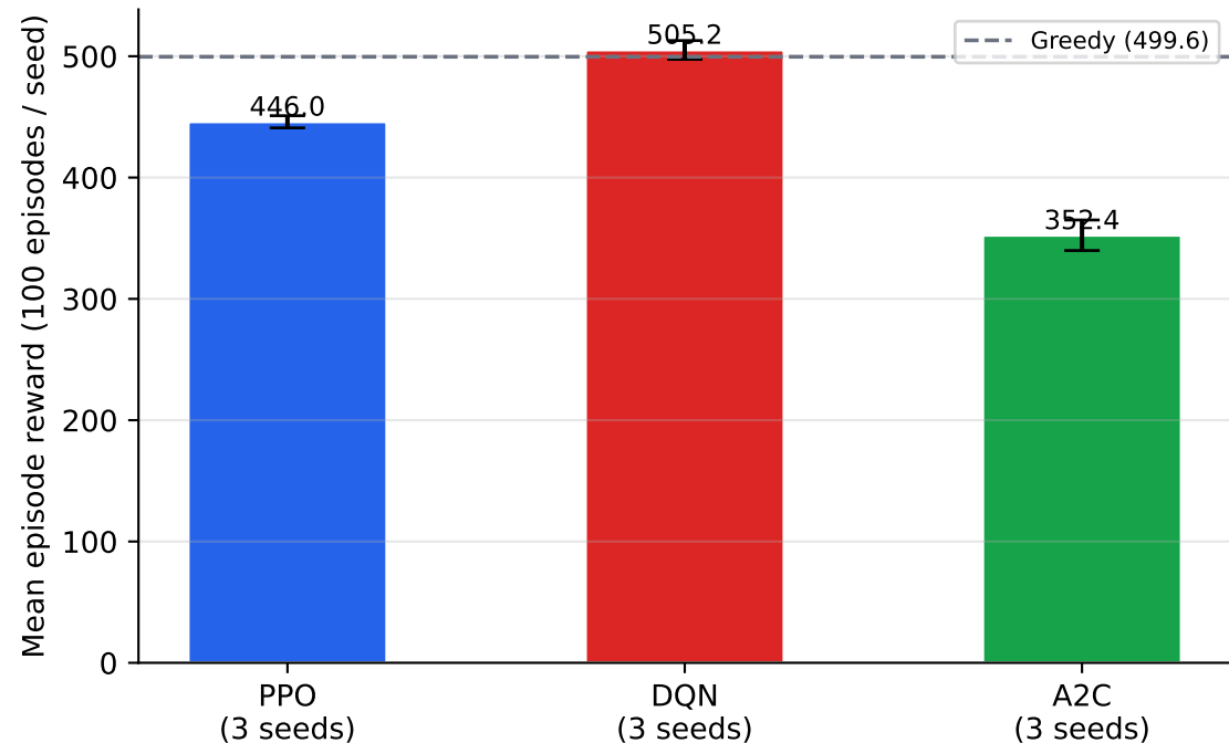
Multi-Seed Robustness Check (seeds=[42, 123, 777], \lambda=3.0 )
