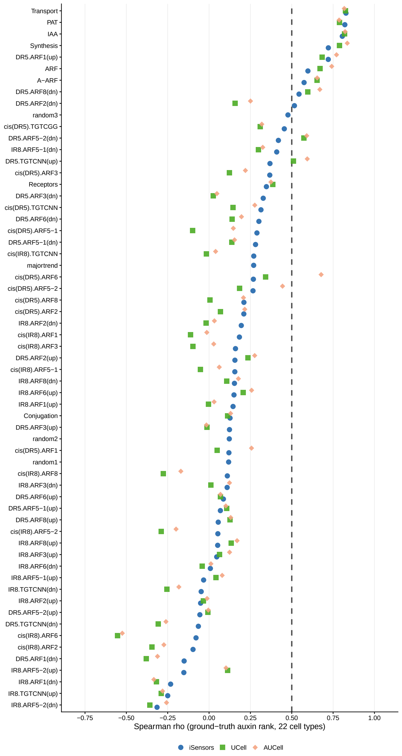
Auxin gradient Spearman rho -- all sensors (groundtruth object)
