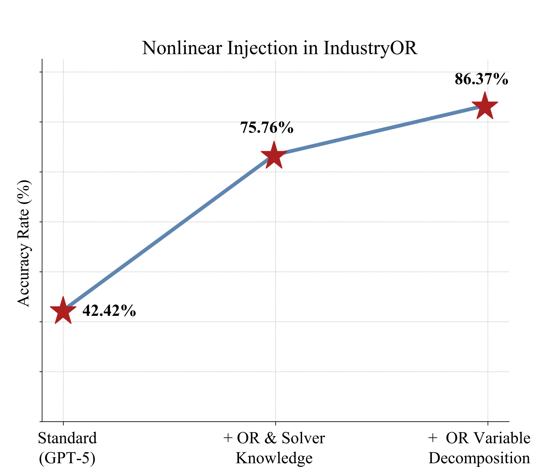
(c) Accuracy of Deeper OR Knowledge
