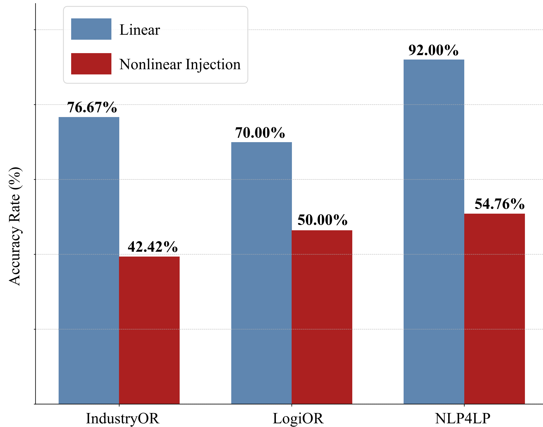
(a) Linear/Nonlinear Injection Average Accuracy
