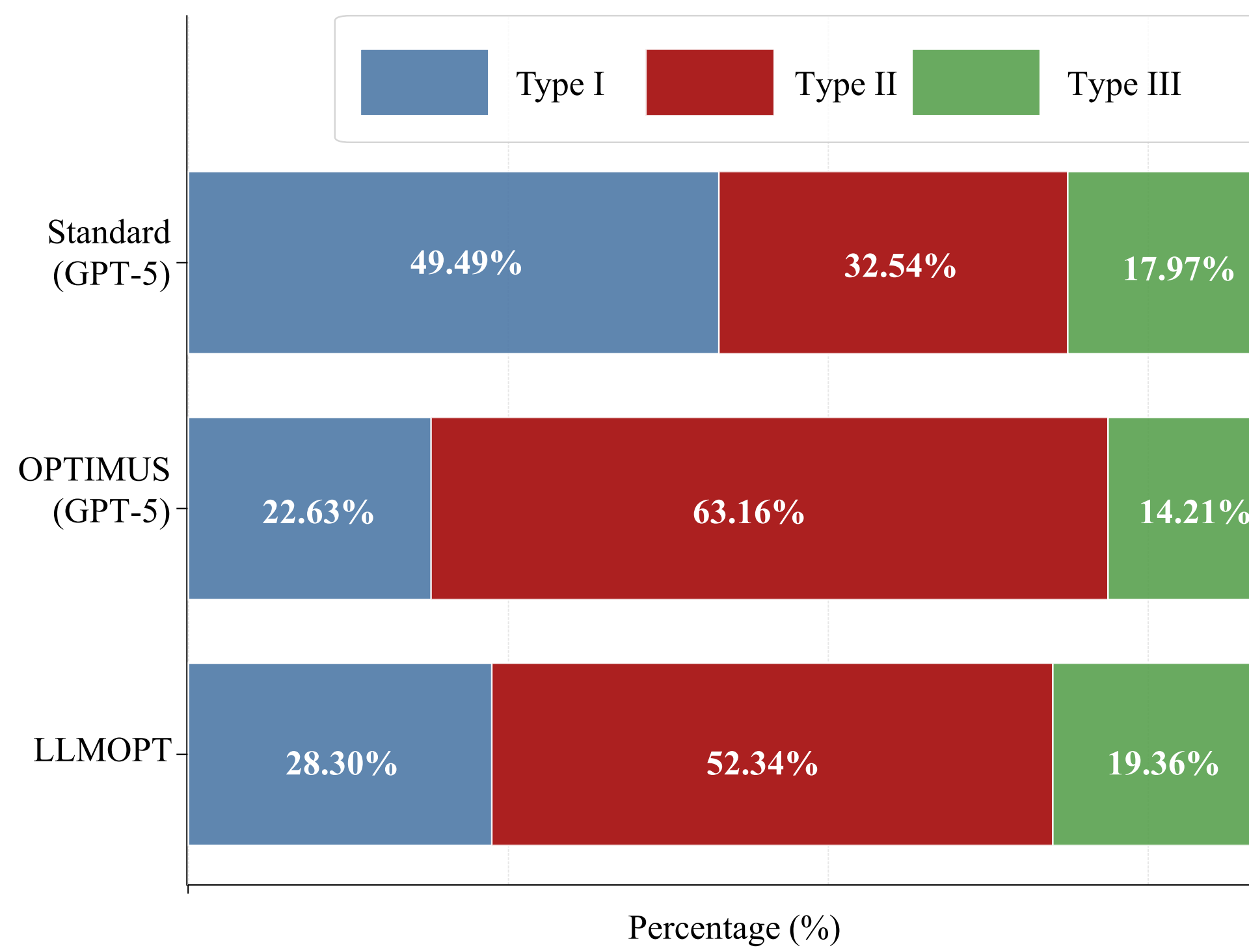
(b) Proportion of 3 Error Types in Nonlinear Injection
