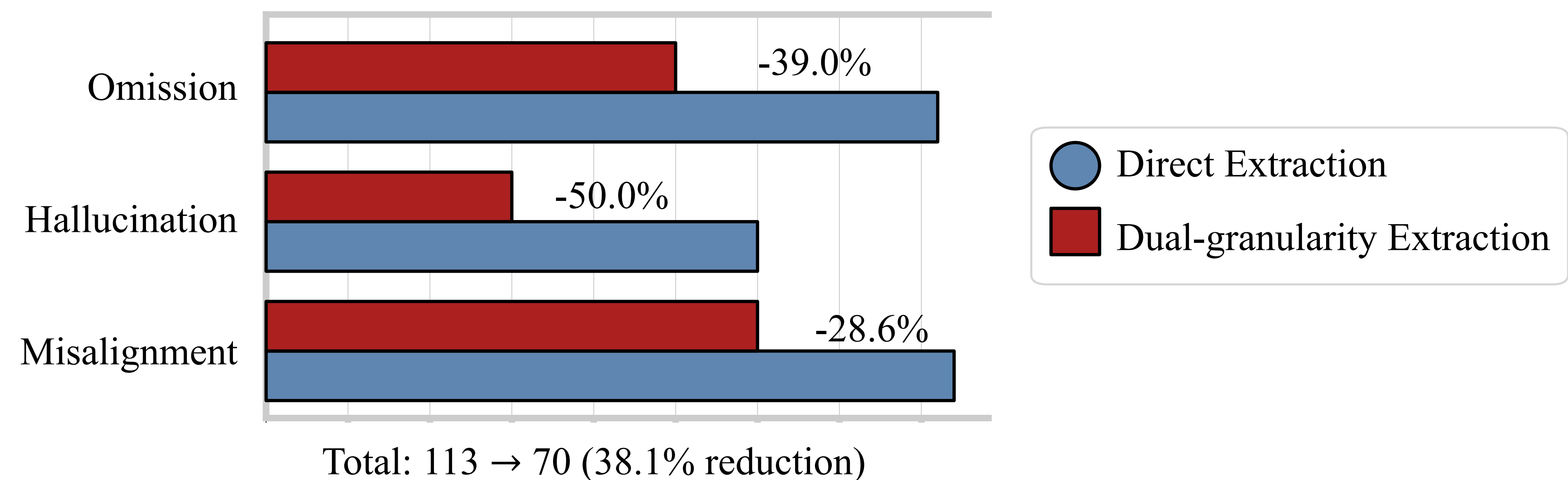
(e) Extraction failure reduction
