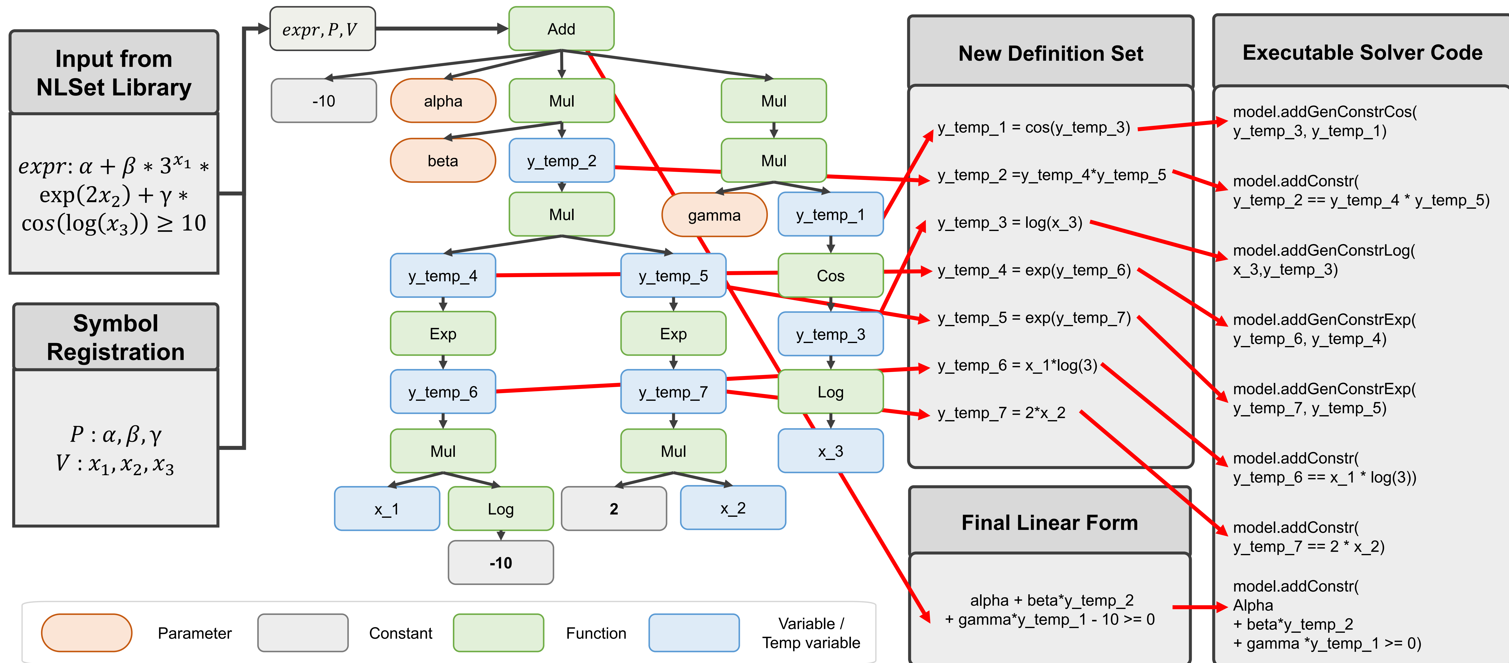
(b) Case study for complex nonlinear expression : \alpha + \beta * 3^{x_1} * \exp(2x_2) + \gamma * \cos(\log(x_3)) \geq 10
