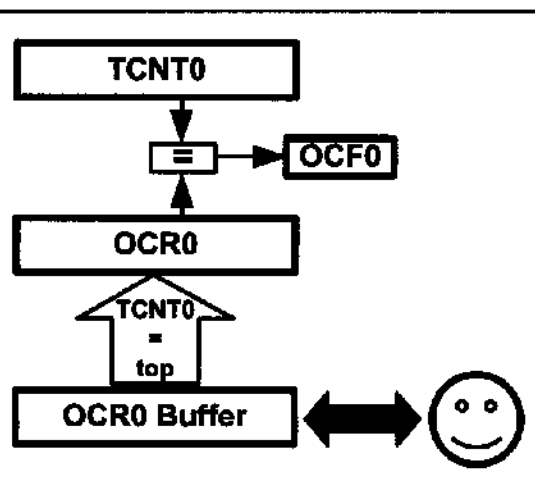
Figure 16-16. OCRn Buffer in PWM Modes
