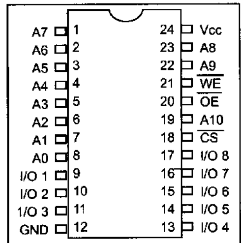
Figure 0-11. 2K x 8 SRAM Pins
