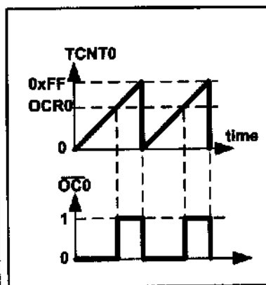
Figure 16-14B. Inverted
