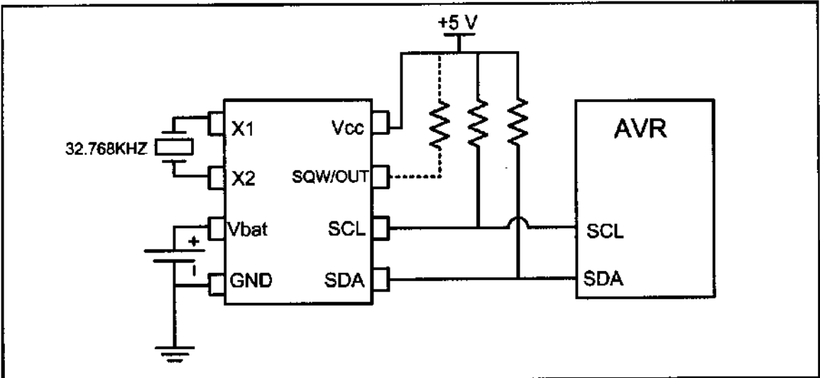
Figure H-9. DS1307 Power Connection Options (Maxim/Dallas Semiconductor)
