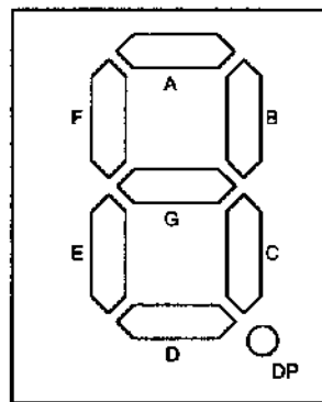
Figure 17-11. 7-segment LEDs
