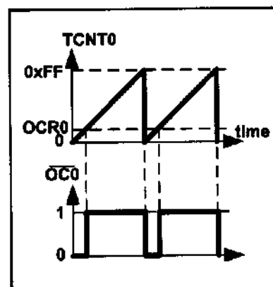
Figure 16-14A. Inverted
