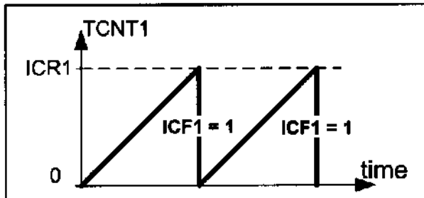
Figure 15-10. Modes 12 and 14
