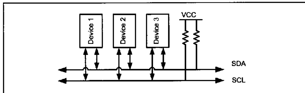
Figure 18-1. I2C Bus
