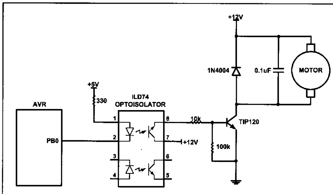
Figure 16-7. DC Motor Connection Using a Darlington Transistor
