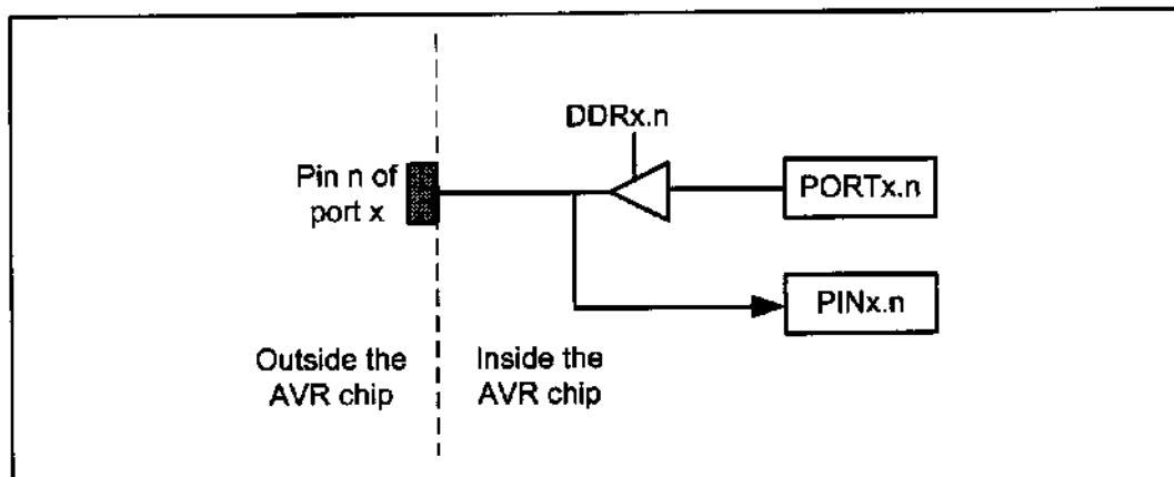
Figure 4-3. The I/O Port in AVR
