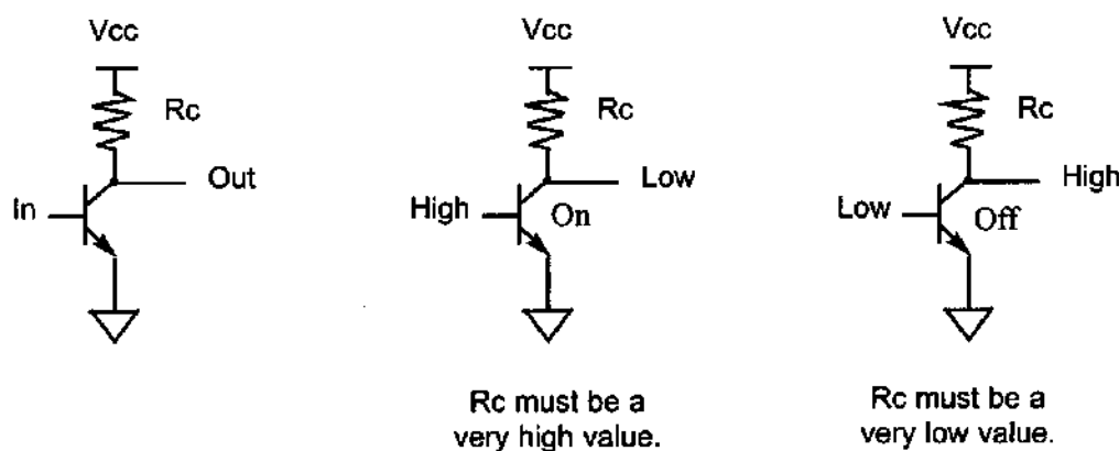
Figure C-2. One-Transistor Inverter with Pull-up Resistor
