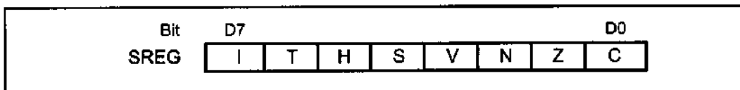
Figure 6-1. Bits of the Status Register
