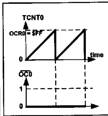
Figure 16-14C. Inverted
