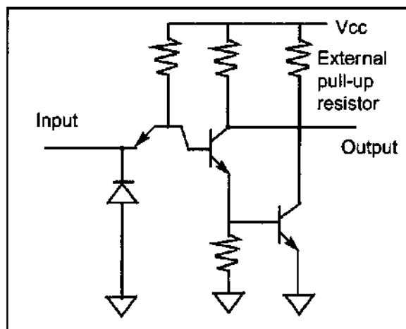
Figure C-5. Open Collector
