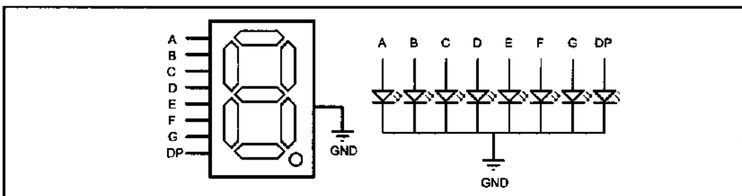
Figure 17-13. Common Cathode Connections in a 7-Segment Display
