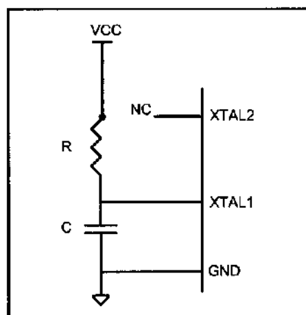
Figure 8-5 External RC
