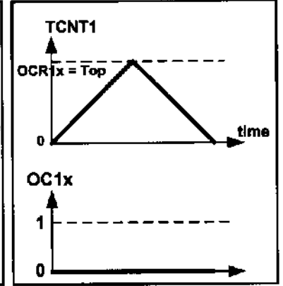
Figure 16-45C. Inverted
