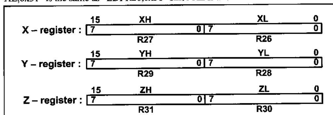
Figure 6-6. Registers X, Y, and Z
