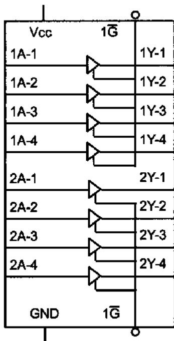
Figure C-8 (a). 74LS244 Octal Buffer
