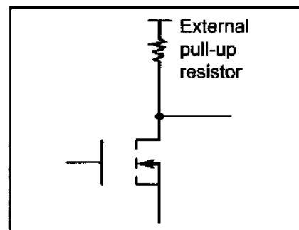
Figure C-6. Open Drain
