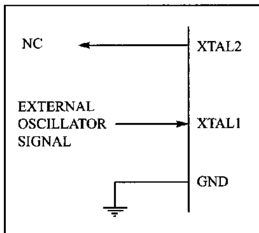
Figure 8-6a. XTAL1 Connection to an External Clock Source
