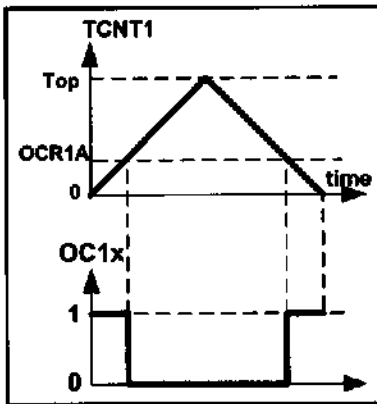
Figure 16-44A. Non-inverted
