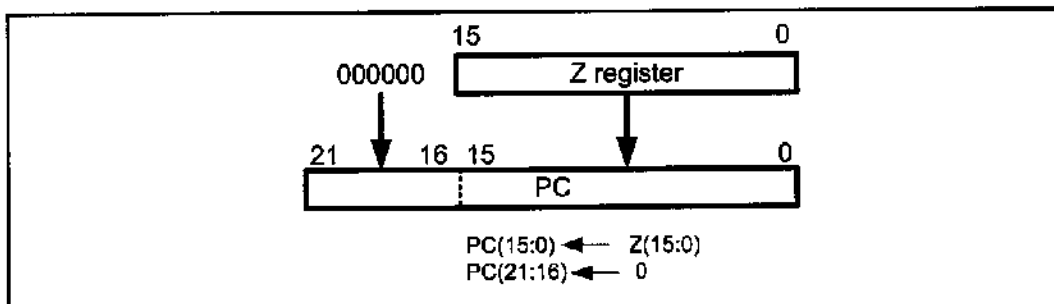
Figure 3-10. ICALL Instruction
