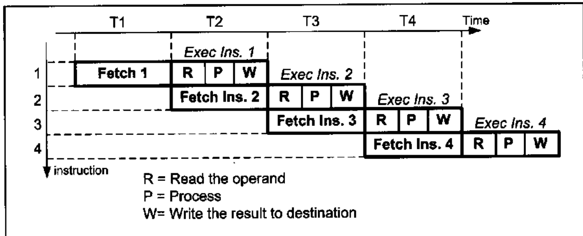
Figure 3-14. Pipeline Activity for Both Fetch and Execute
