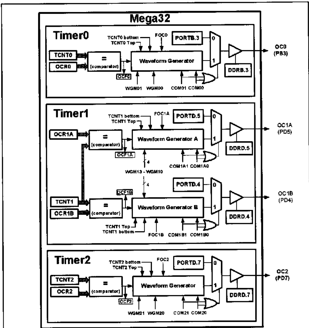
Figure 15-12. Waveform Generators in ATmega32
