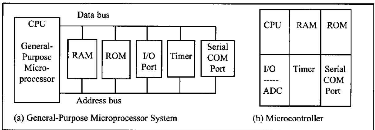
Figure 1-1. Microprocessor System Contrasted with Microcontroller System
