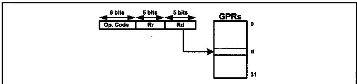
Figure 6-3. Two-Register Addressing
