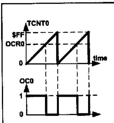
Figure 16-13B. Non-inverted
