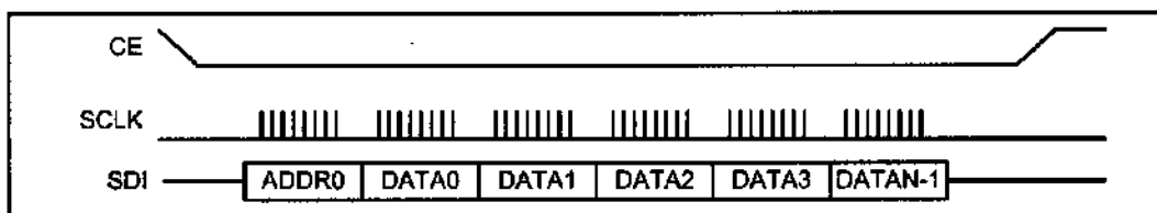
Figure 17-5. SPI Burst (Multibyte) Mode Writing
