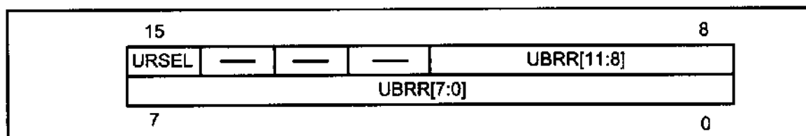
Figure 11-10. UBRR Register
