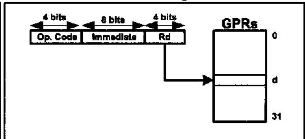
Figure 6-2b. Single-Register (with immediate)
