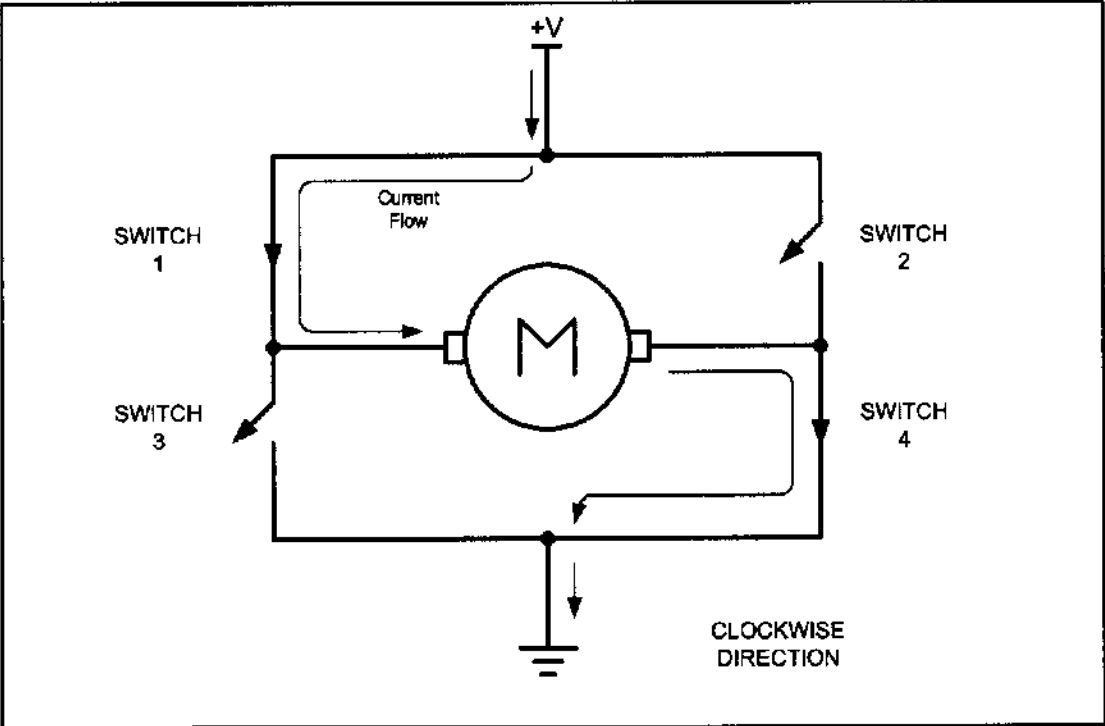
Figure 16-3. H-Bridge Motor Clockwise Configuration
