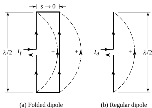
Figure 9.16 Folded dipole and equivalent regular dipole.
