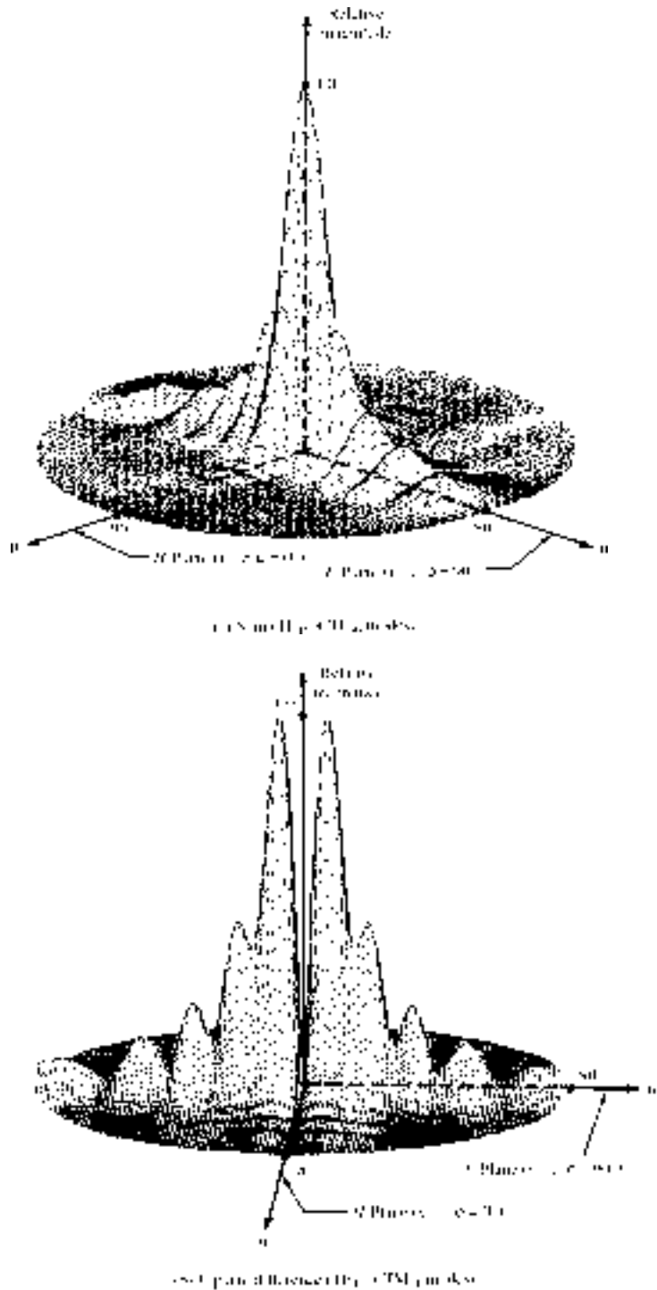
Figure 13.35 Three-dimensional sum and difference ( E - and H -planes) field patterns of a monopulse pyramidal horn. (SOURCE: C. A. Balanis, "Horn Antennas," in Antenna Handbook (Y. T. Lo and S. W. Lee, eds.), © 1988, Van Nostrand Reinhold Co., Inc.)
