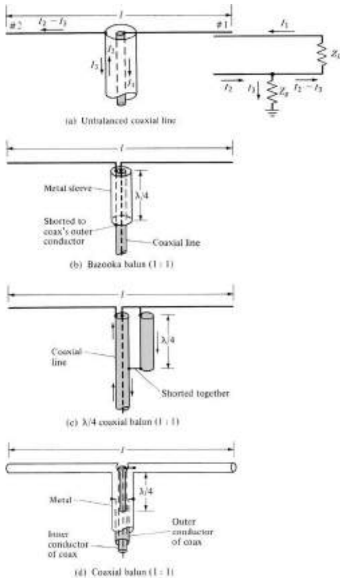
Figure 9.25 Balun configurations.
