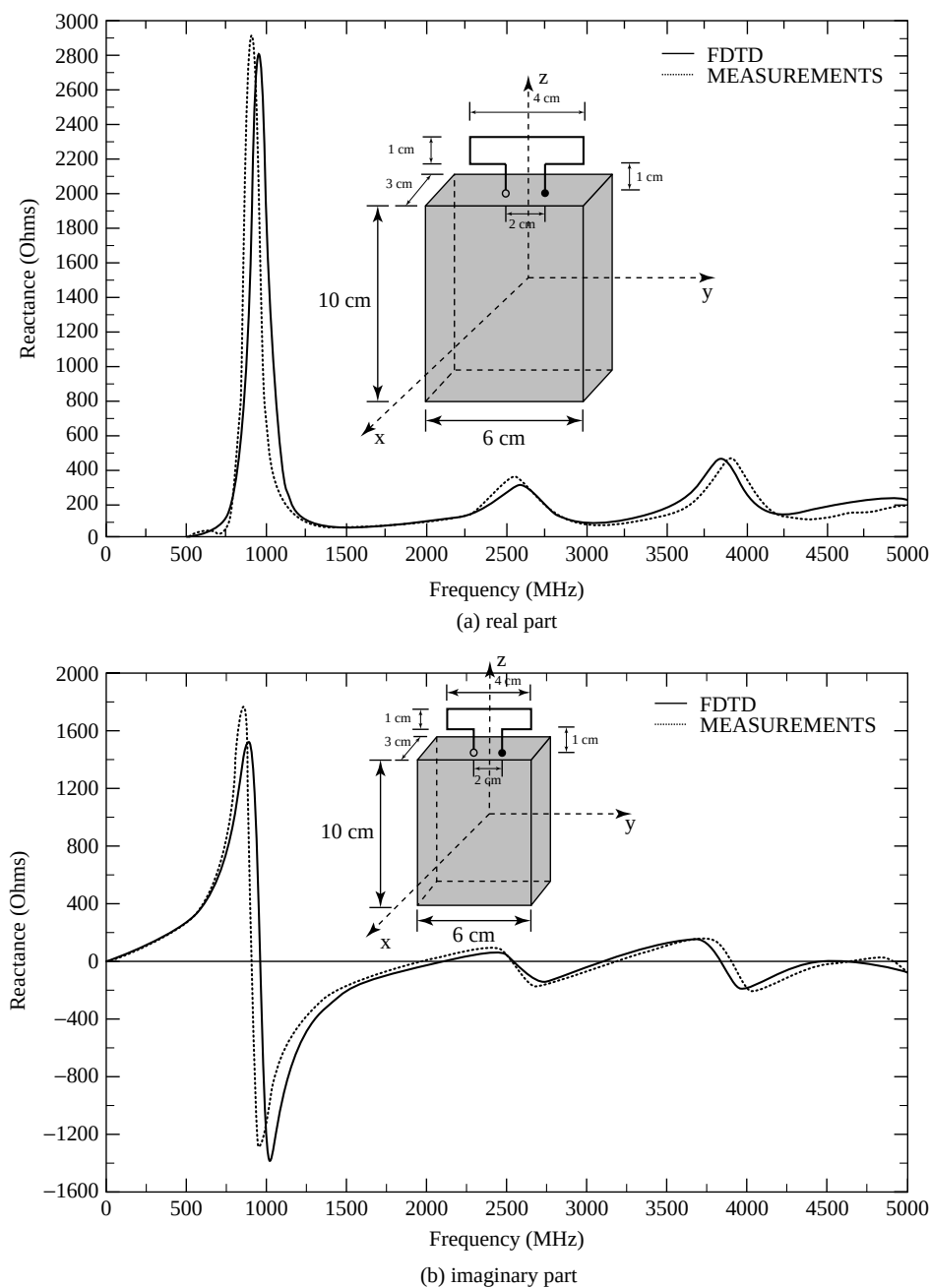
Figure 5.20 Input impedance, real and imaginary parts of a wire folded loop mounted vertically on a conducting mobile hand-held unit (SOURCE: K. D. Katsibas, et. al., “Folded Loop Antenna for Mobile Hand-Held Units,” IEEE Transactions Antennas Propagat. , Vol. 46, No. 2, February 1998, pp. 260–266. © 1998 IEEE).
