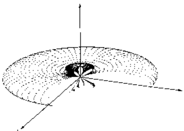
Figure 6.6a (broadside) ( \beta = 0, d = \lambda/4 )
