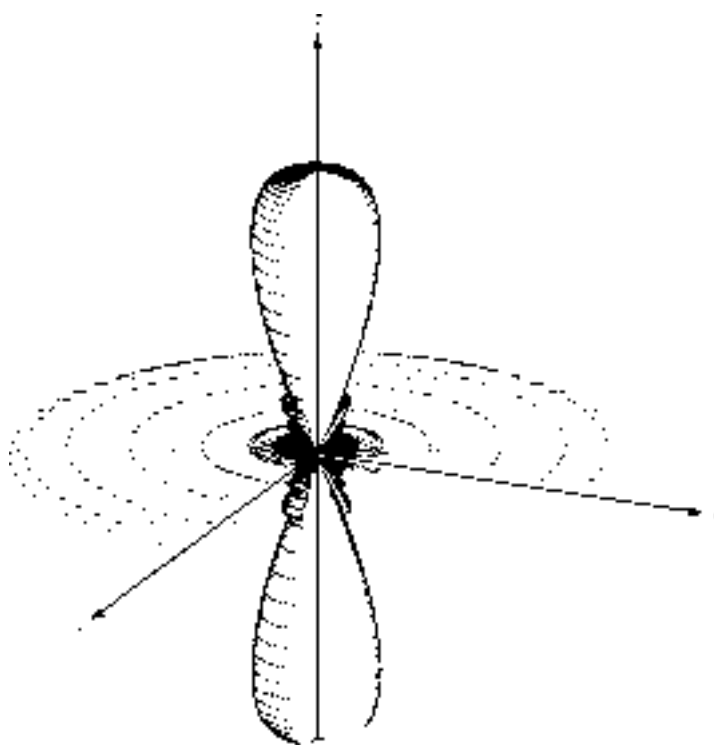
Figure 6.6b (broadside/end-fire) ( \beta = 0, d = \lambda )
