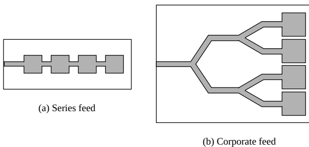
Figure 14.36 Feed arrangements for microstrip patch arrays.
