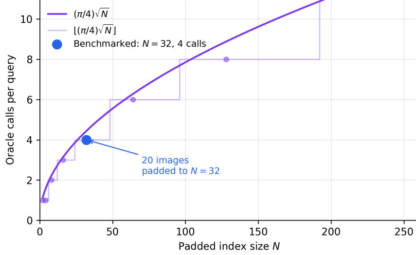
Figure 7: Theoretical Grover oracle-call count \lfloor (\pi/4)\sqrt{N} \rfloor as a function of the padded index size N , with a marker at the single size we benchmarked ( N = 32 , four oracle calls). We ran one dataset size, so this confirms the count at a single point on the curve rather than tracing the curve empirically.
