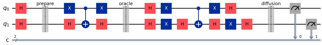
Figure 6: One Grover iteration for a four-element index ( N = 4 , two index qubits). After preparing a uniform superposition, the oracle flips the phase of the marked index and the diffusion operator amplifies its amplitude; the two qubits are then measured. The barriers separate the preparation, oracle, and diffusion phases.
