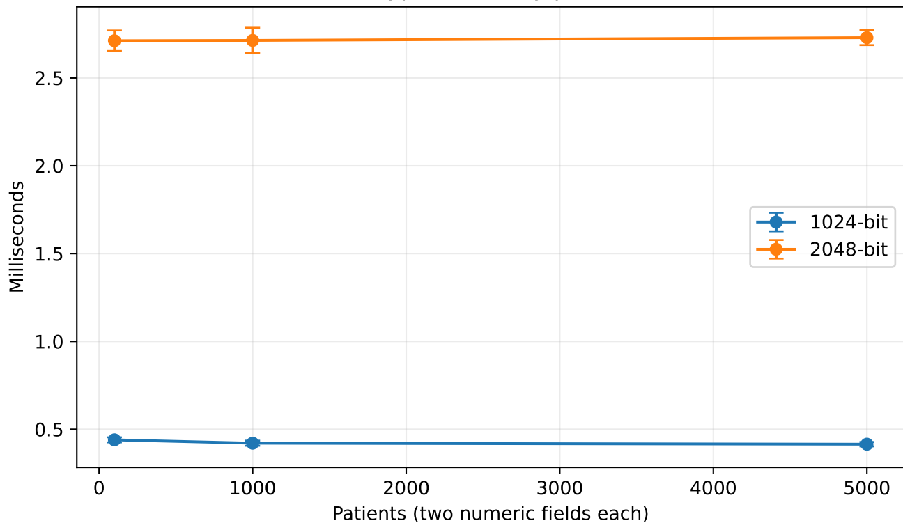
Decryption latency per field
