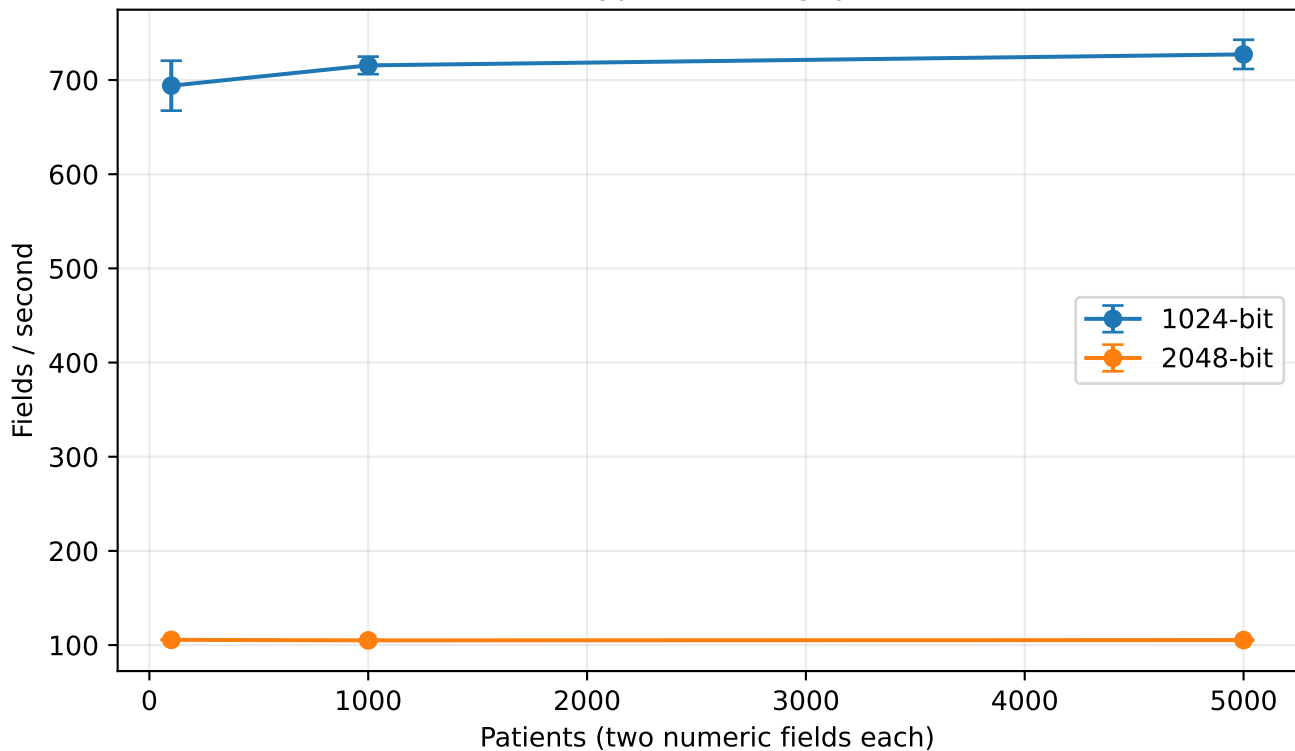
Encryption throughput
