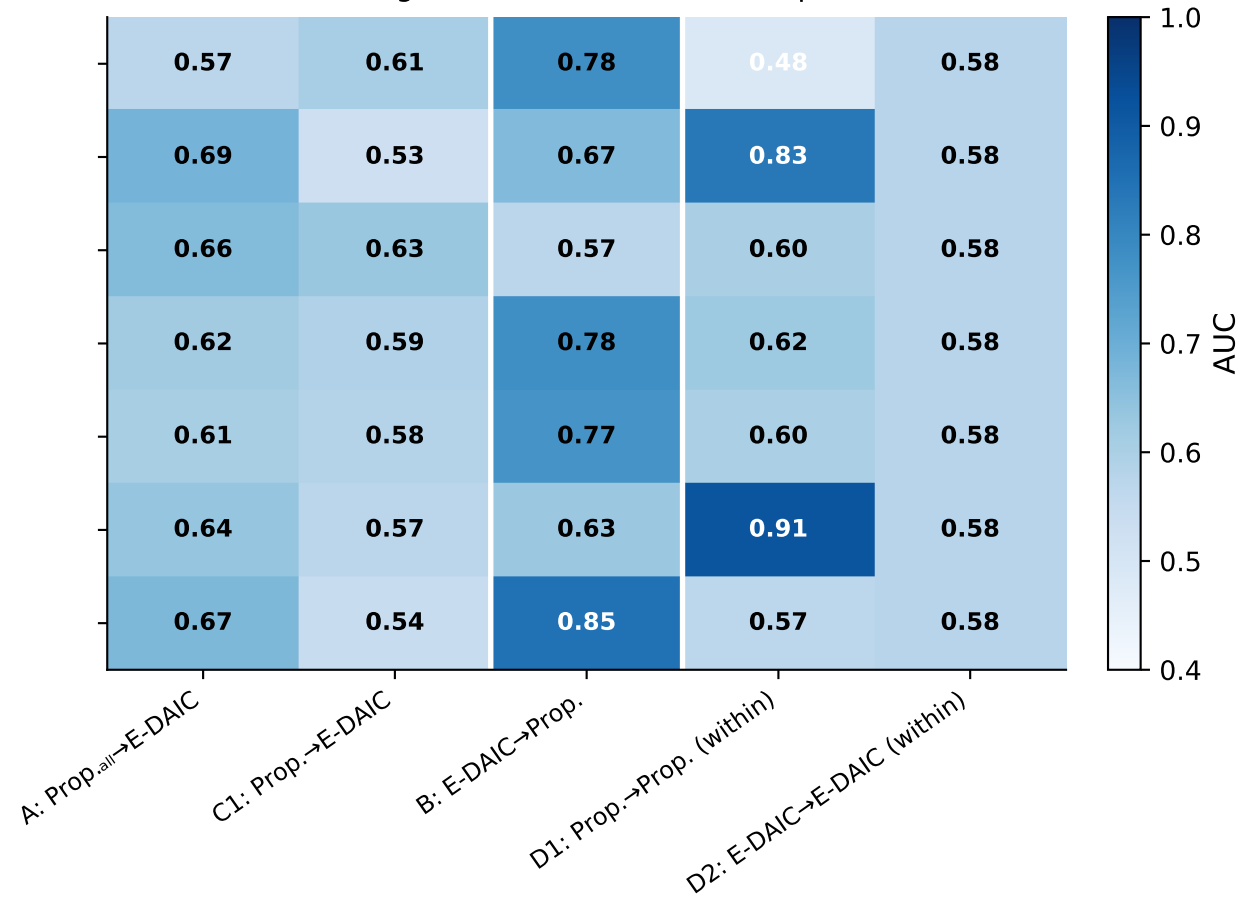
Setting 2: PHQ-8 \geq 10 for both corpora
