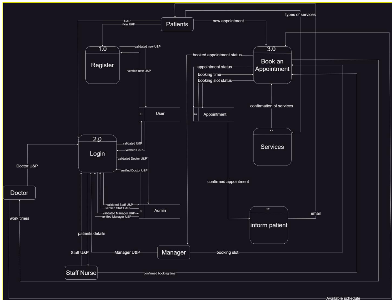
Figure 4.2.1.1(b): Level 0 of Booking Appointment System
