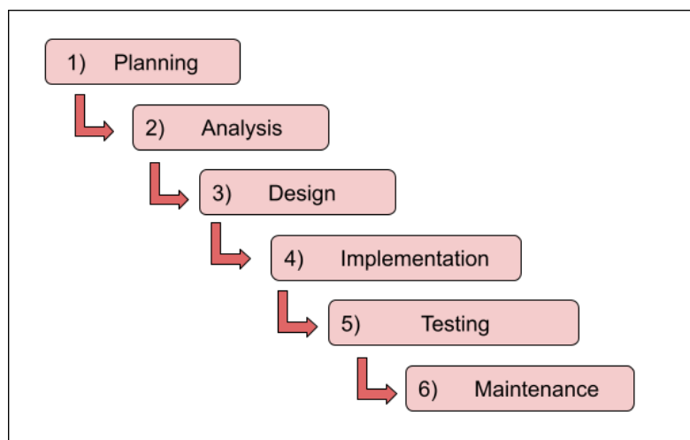
Figure 3.1: Waterfall Model
