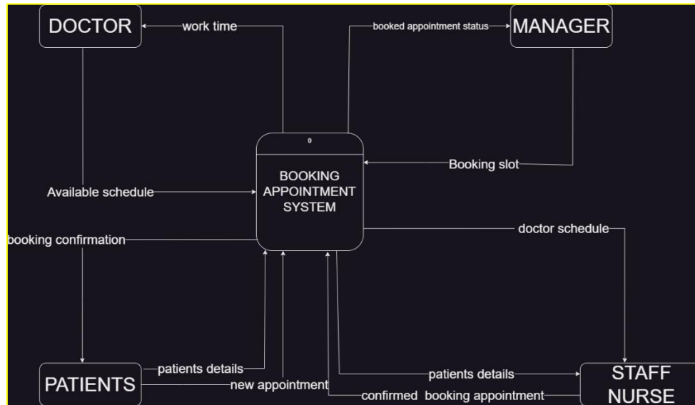
Figure 4.2.1.1(a): Context Diagram of Booking Appointment System
