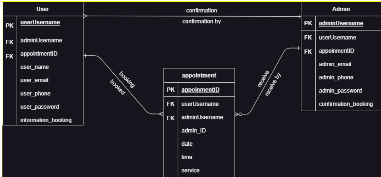
Figure 4.3.1(a): ERD Diagram
