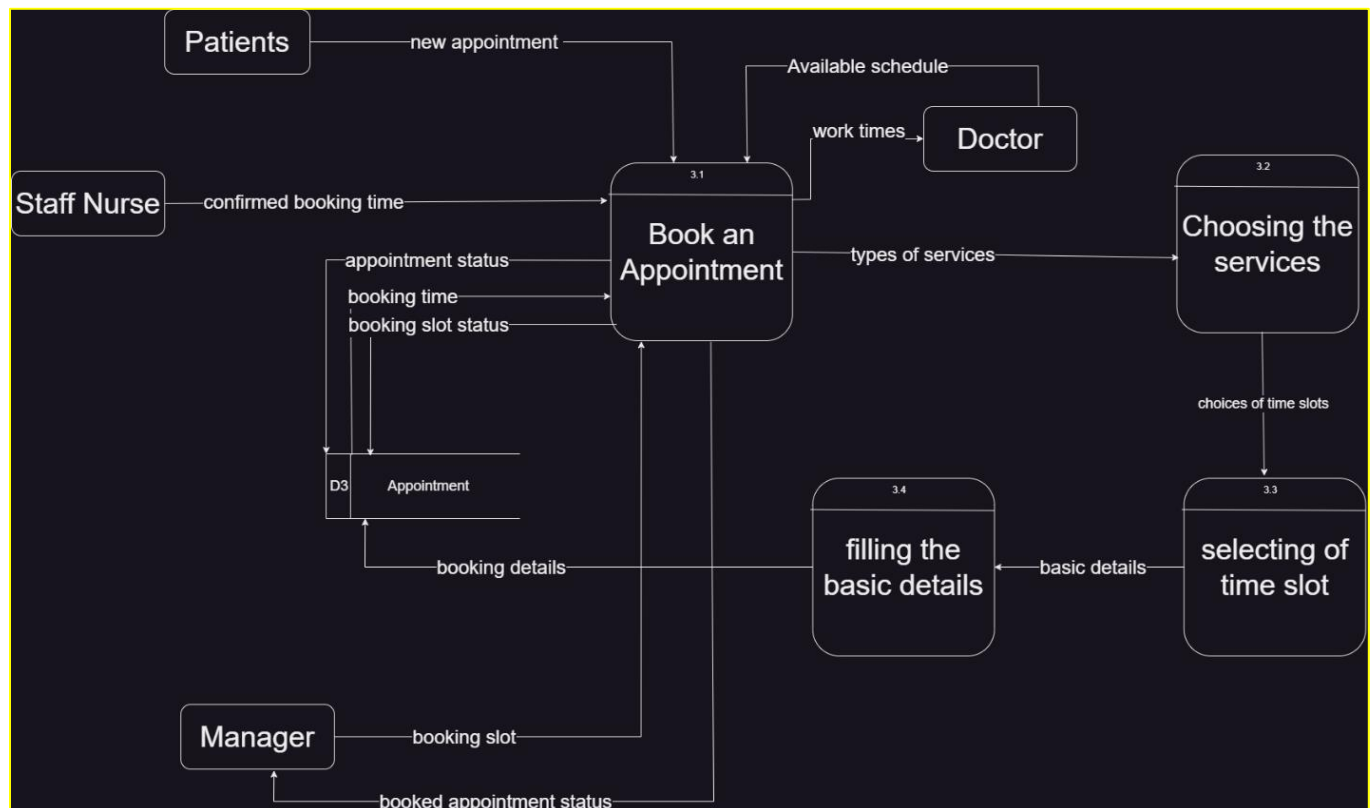
Figure 4.2.1.1(c): Level 1 of Booking an Appointment Process
