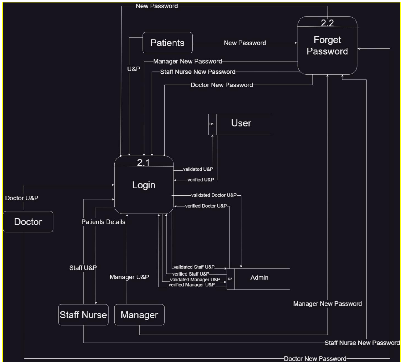
Figure 4.2.1.1(b): Level 1 of Login Process
