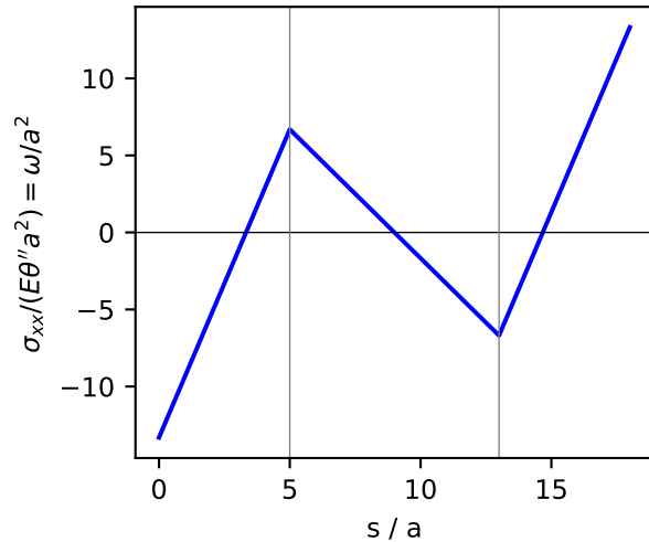
constrained warping normal stress \sigma_{xx}(s) (and u(s) \propto \omega )
