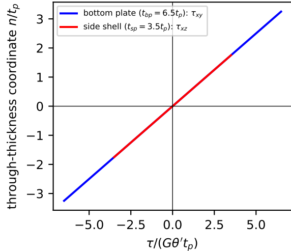
free warping (St. Venant) shear stress
