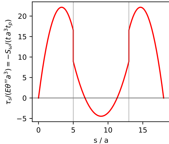
constrained warping shear stress \tau(s) = -E\theta'''S_\omega/t
