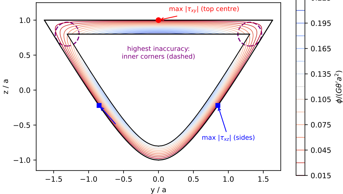
Prandtl function \phi/(G\theta'a^2) of the solid section, plotted in the wall ( c = a , k = 0.8 )
