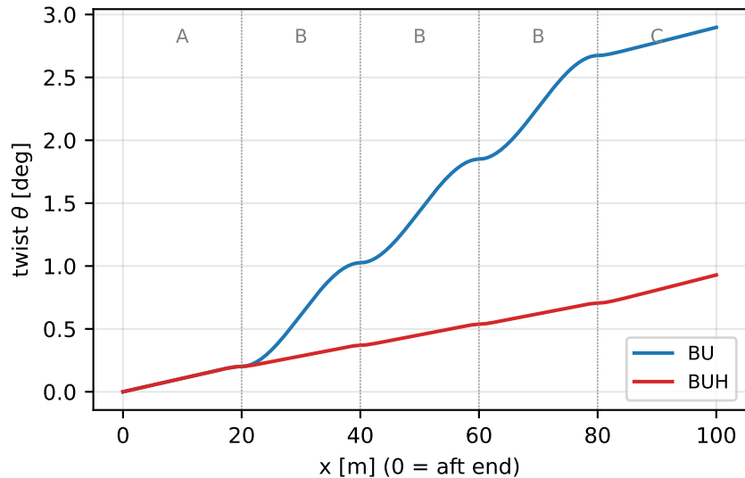
rotation \theta(x) , M_t = 100 MNm
