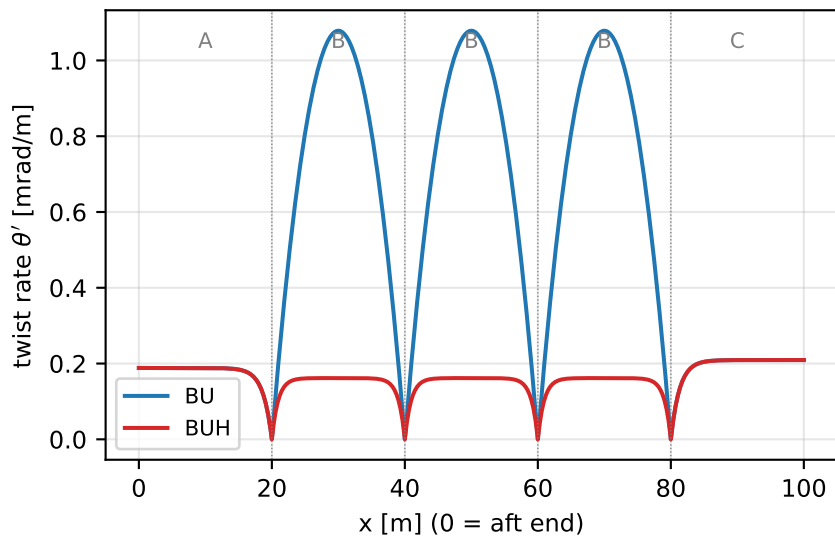
twist rate \theta'(x)
