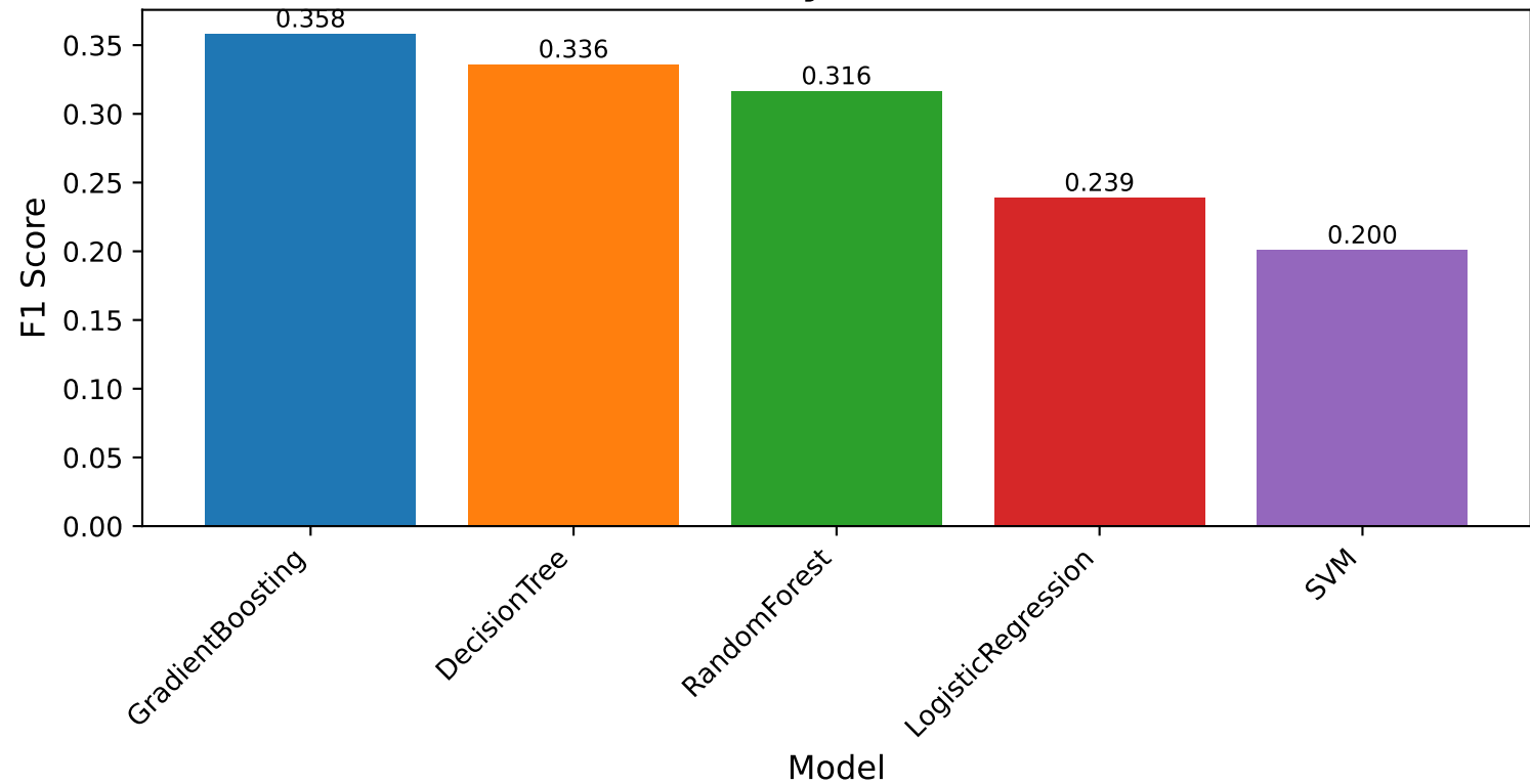
Edu-Primary: Model vs F1
