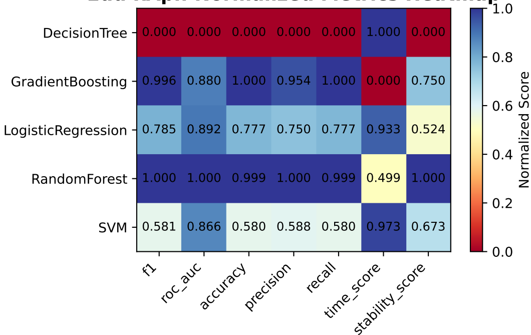
Edu-xApi: Normalized Metrics Heatmap
