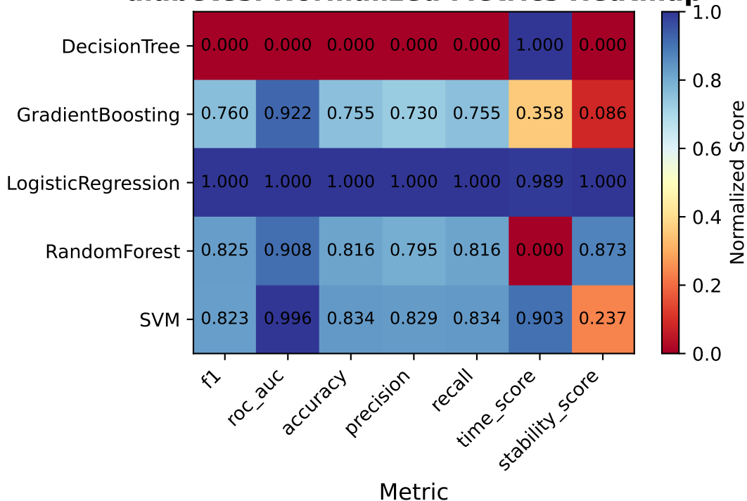
diabetes: Normalized Metrics Heatmap
