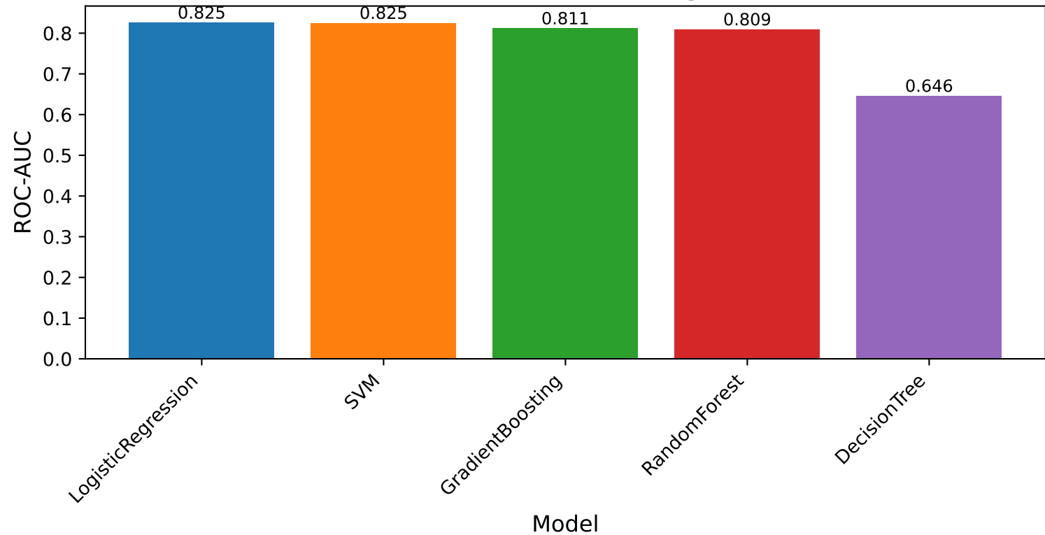
diabetes: ROC-AUC Comparison
