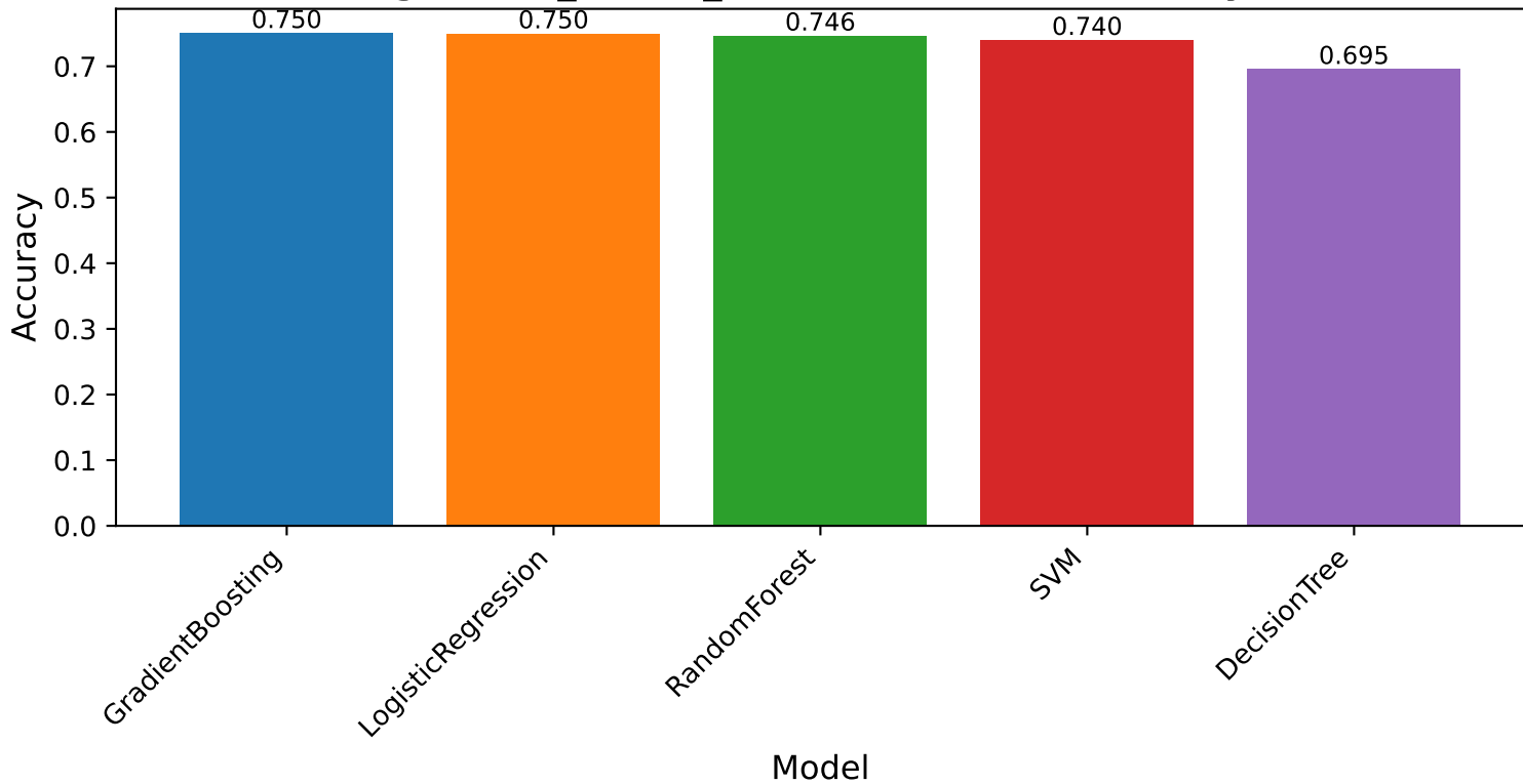
german_credit_data: Model vs Accuracy
