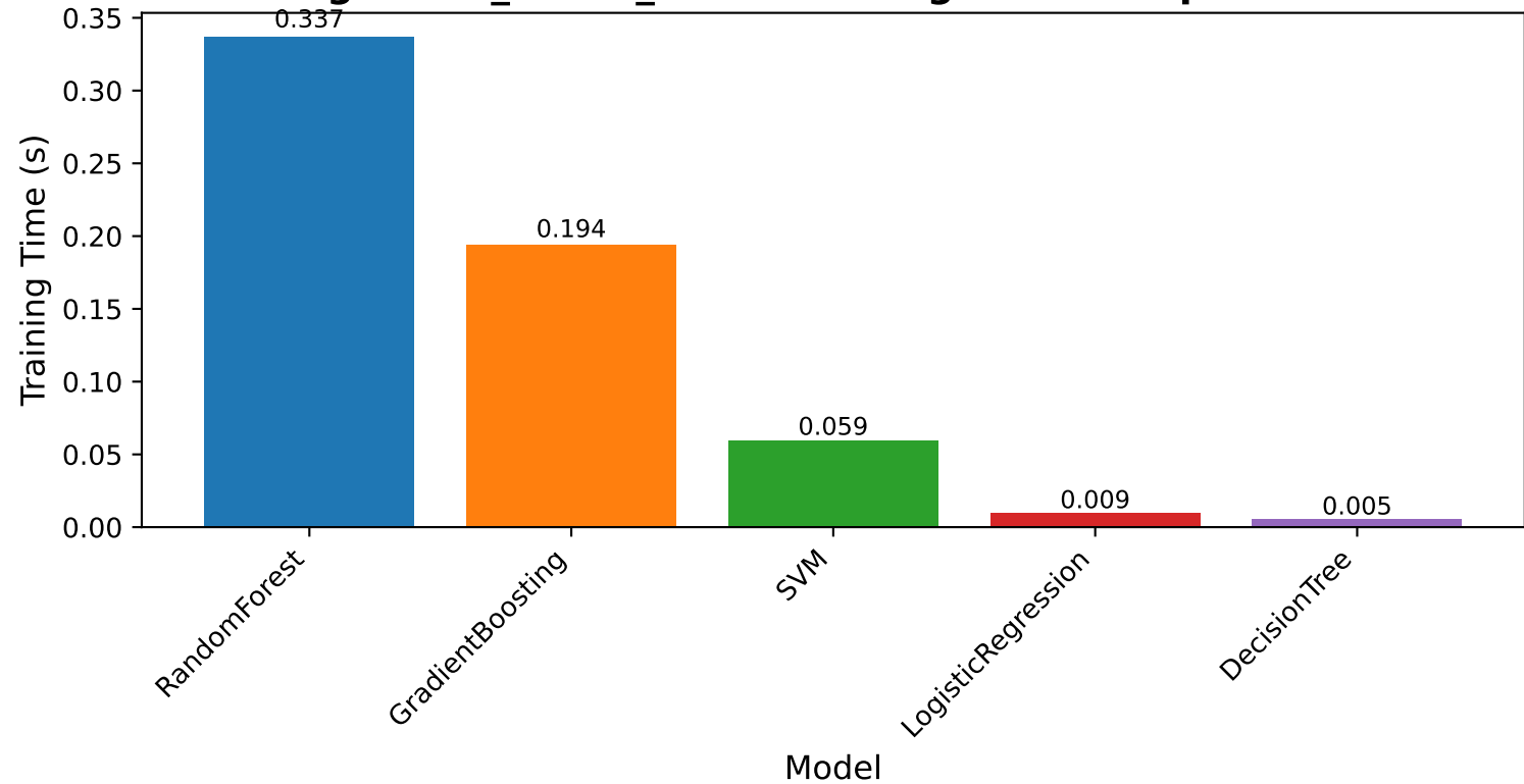
german_credit_data: Training Time Comparison
