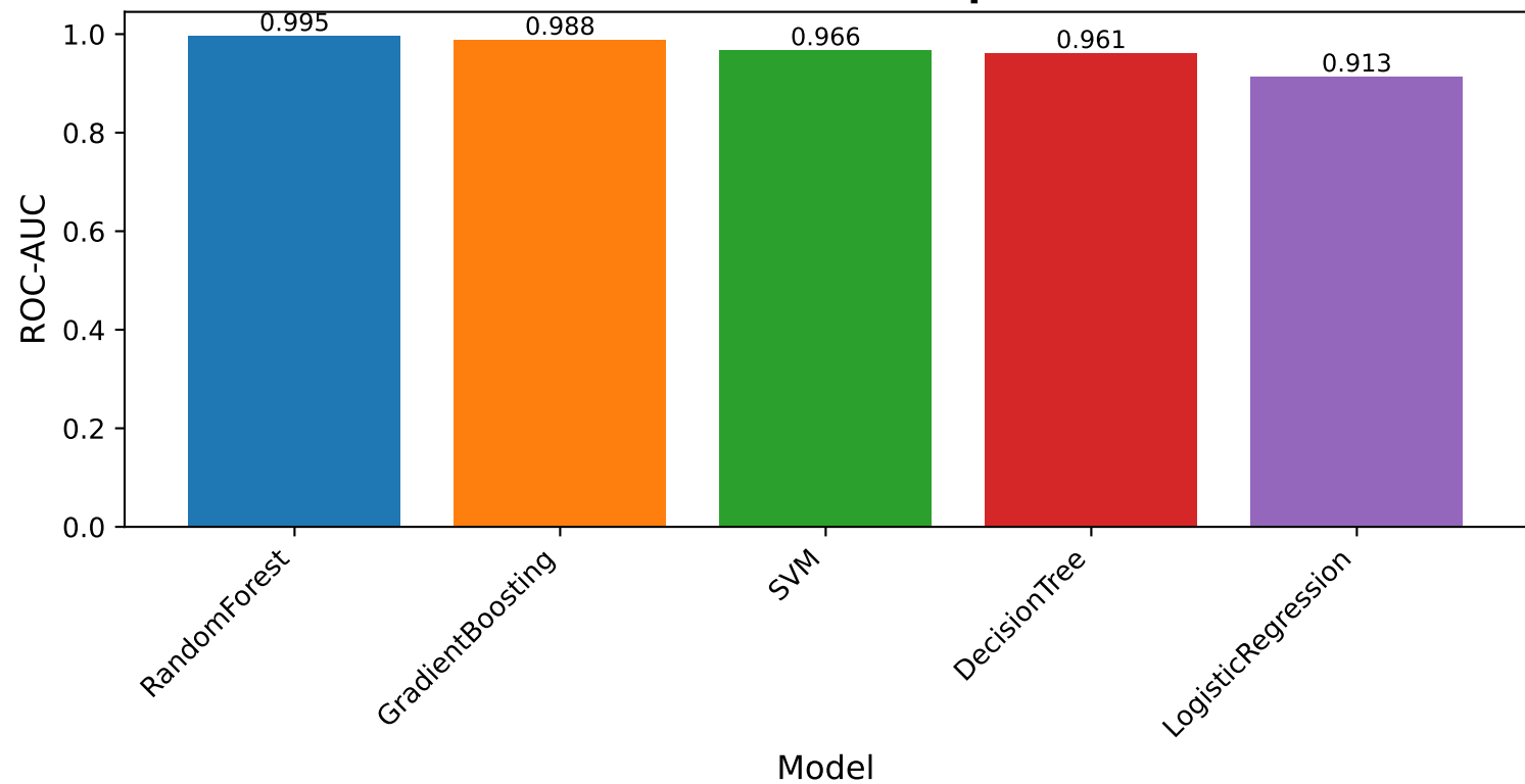
heart: ROC-AUC Comparison
