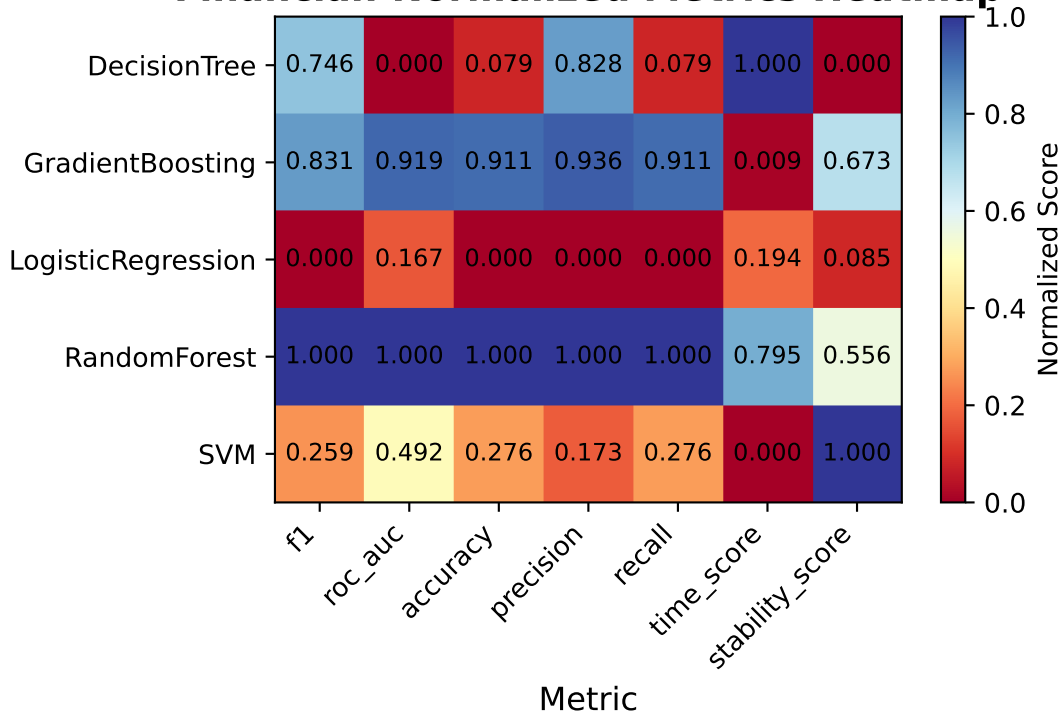
Financial: Normalized Metrics Heatmap
