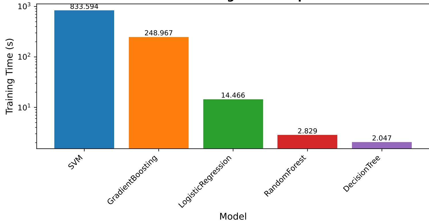
Financial: Training Time Comparison
