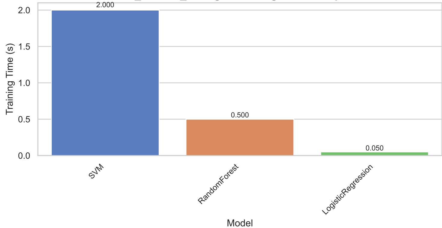
demo_dataset_storage: Training Time Comparison
