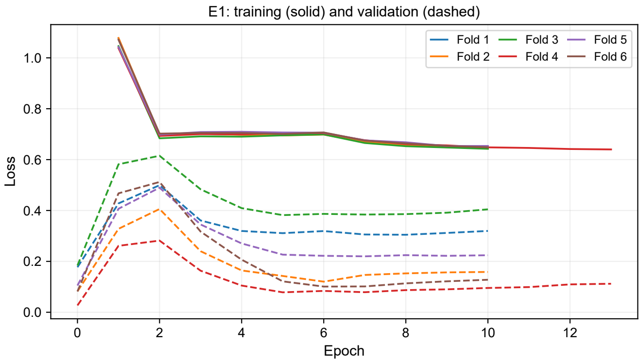
Figure 16: E1: training loss (solid) and validation gallery loss (dashed), all six folds on one set of axes. Most folds recover from the early perturbation; the selected epoch is 5 in five folds and 8 in fold 4.
