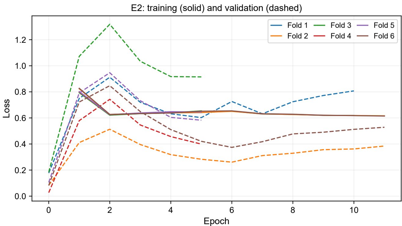
Figure 17: E2: both losses on the same axes, with colour identifying the fold. Greater variability and persistent validation loss accompany epoch-0 selection in three folds. The two loss definitions differ as explained in Section 10.6.
