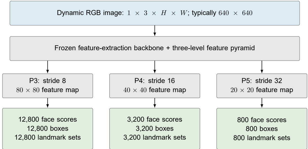
Figure 12: RetinaFace detection architecture: three output scales, each with classification, box regression and landmark heads.
