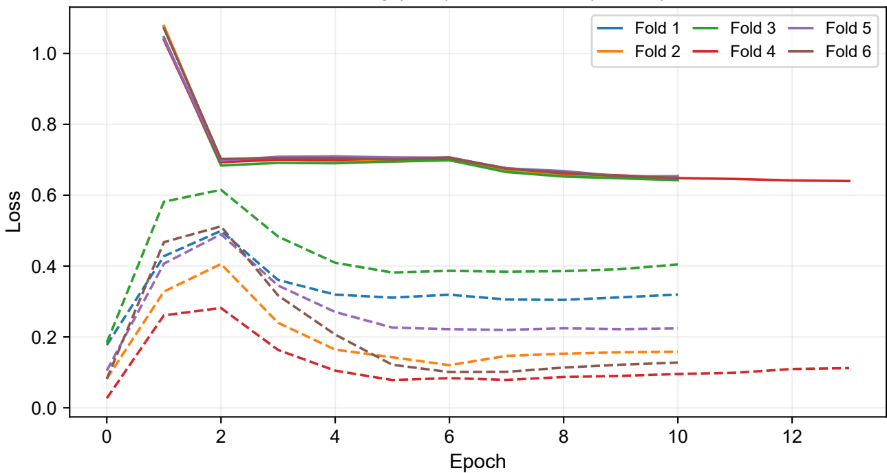
E1: training (solid) and validation (dashed)
