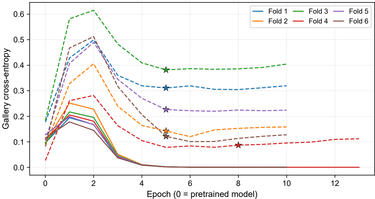
E1: training people (solid) and validation people (dashed)
