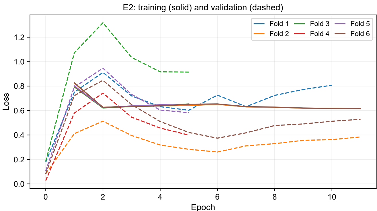
Figure 17: E2: both losses on the same axes, with colour identifying the fold. Greater variability and persistent validation loss accompany epoch-0 selection in three folds. The two loss definitions differ as explained in Section 10.6.
