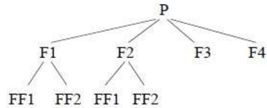
Process Tree
