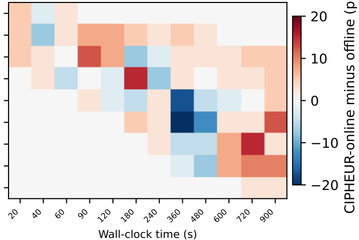
CIPHEUR-online – CIPHEUR-off-VAL
