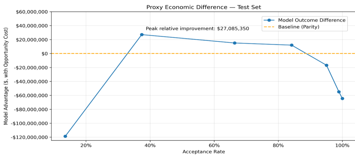
Model vs Baseline — Proxy Economic Comparison Top operating points ranked by model advantage (proxy value with opportunity cost)
